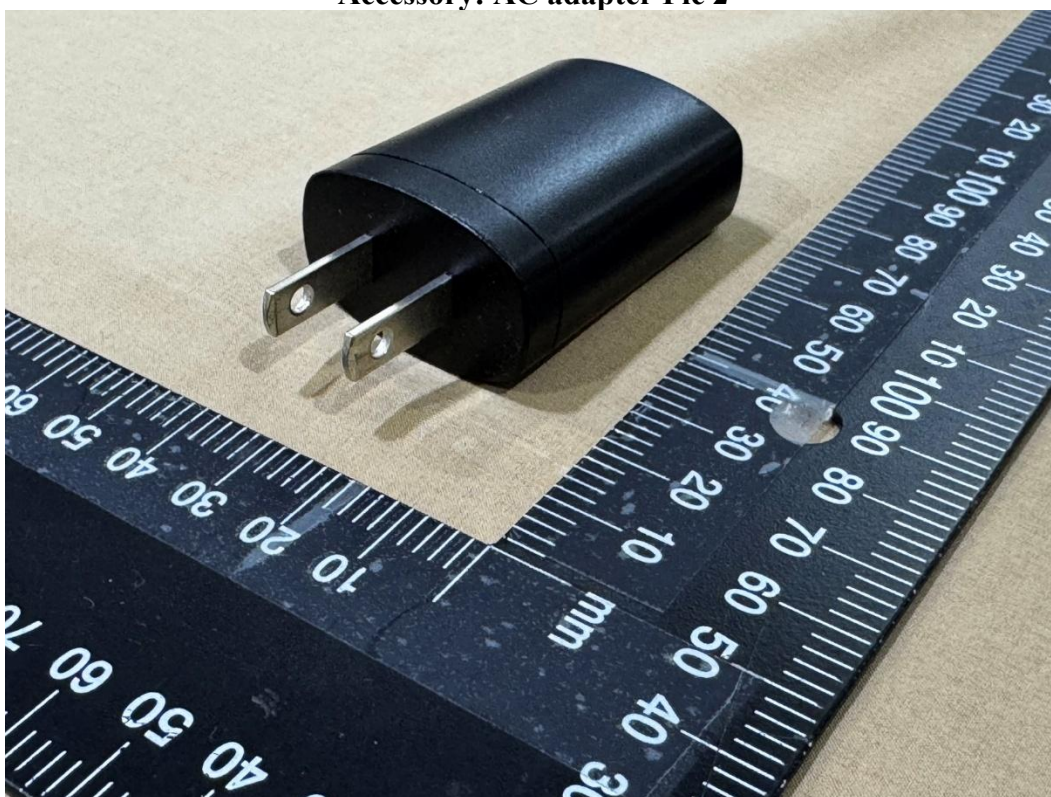
Accessory: AC adapter Pic 2
