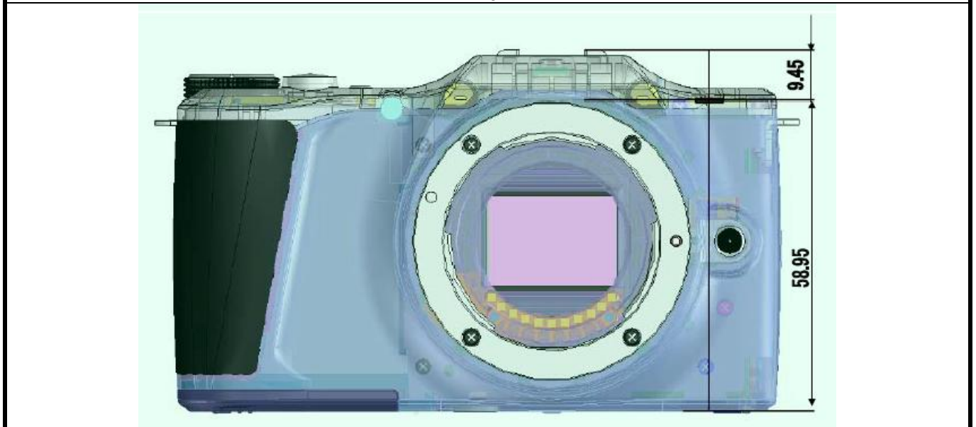
EUT Front View
