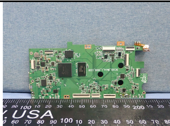
Rear Face of EUT
