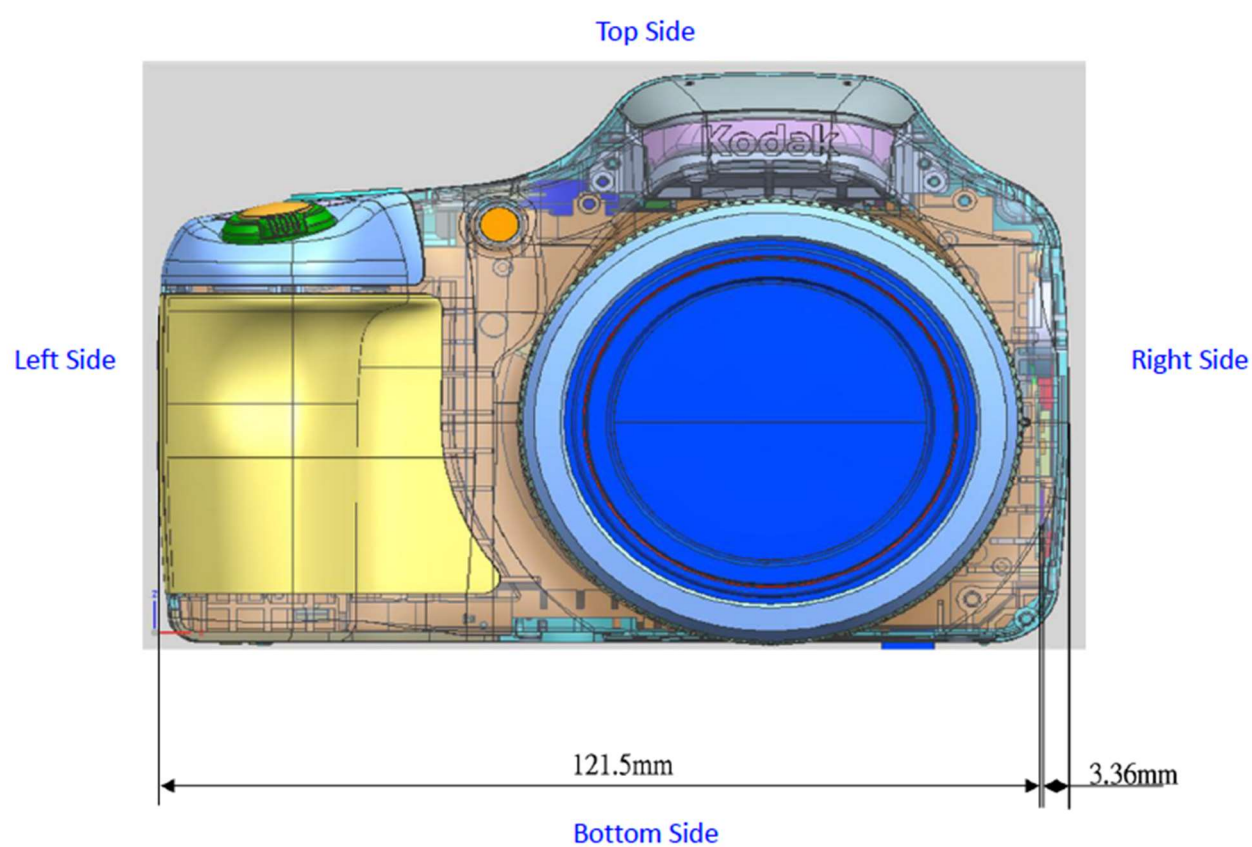
<Front Face View>
