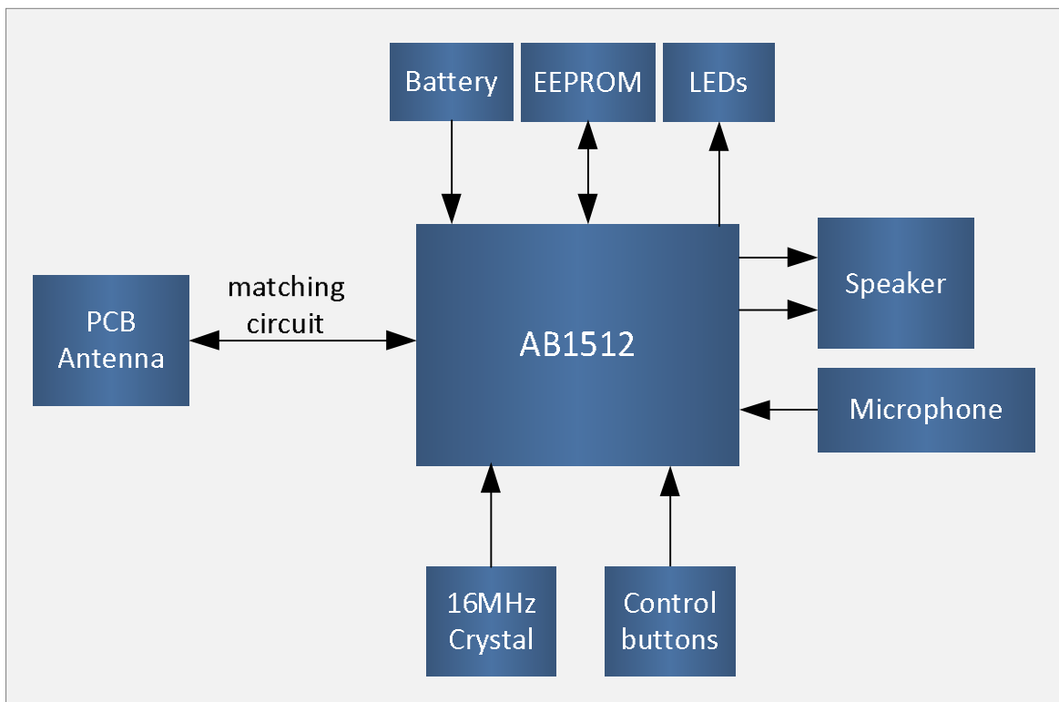
Figure 1-1 Stereo Headset Application Block Diagram
