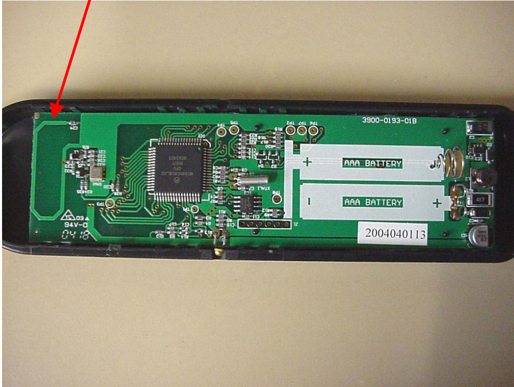
Antenna Location
