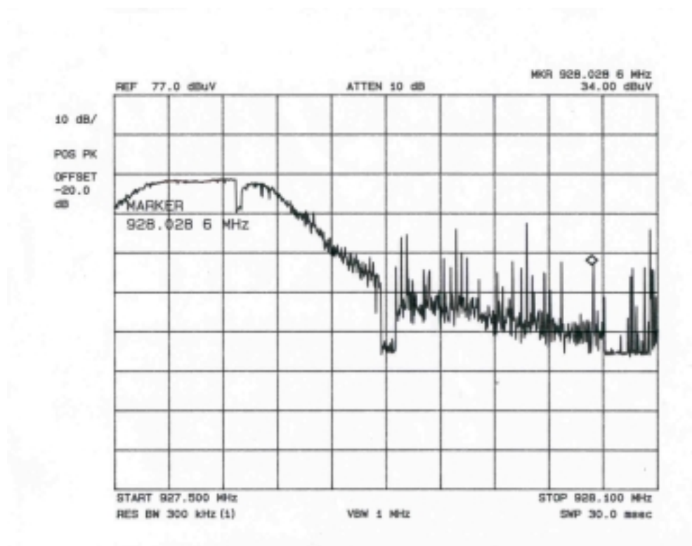
High Channel Bandedge – All Channel Hopping Plot
