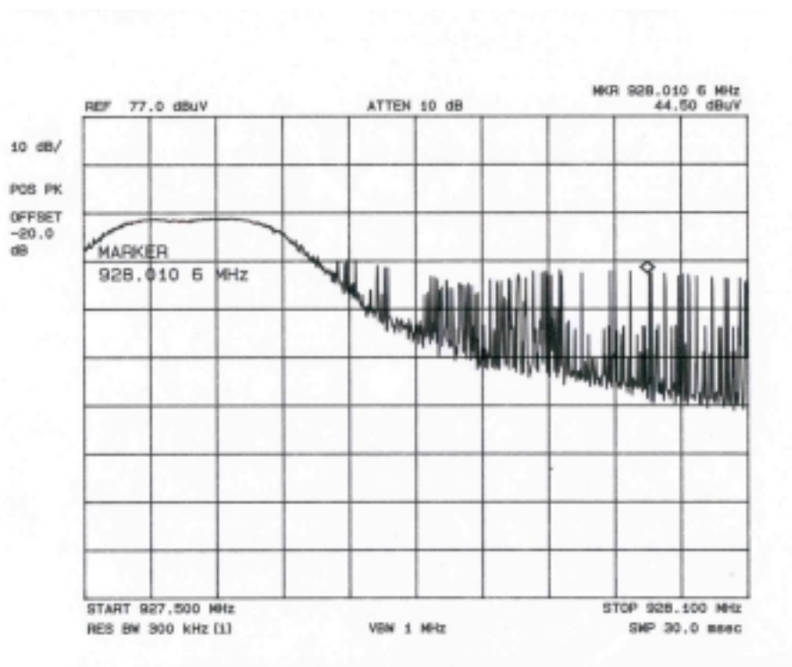
High Channel Bandedge – 2 Channel Hopping Plot
