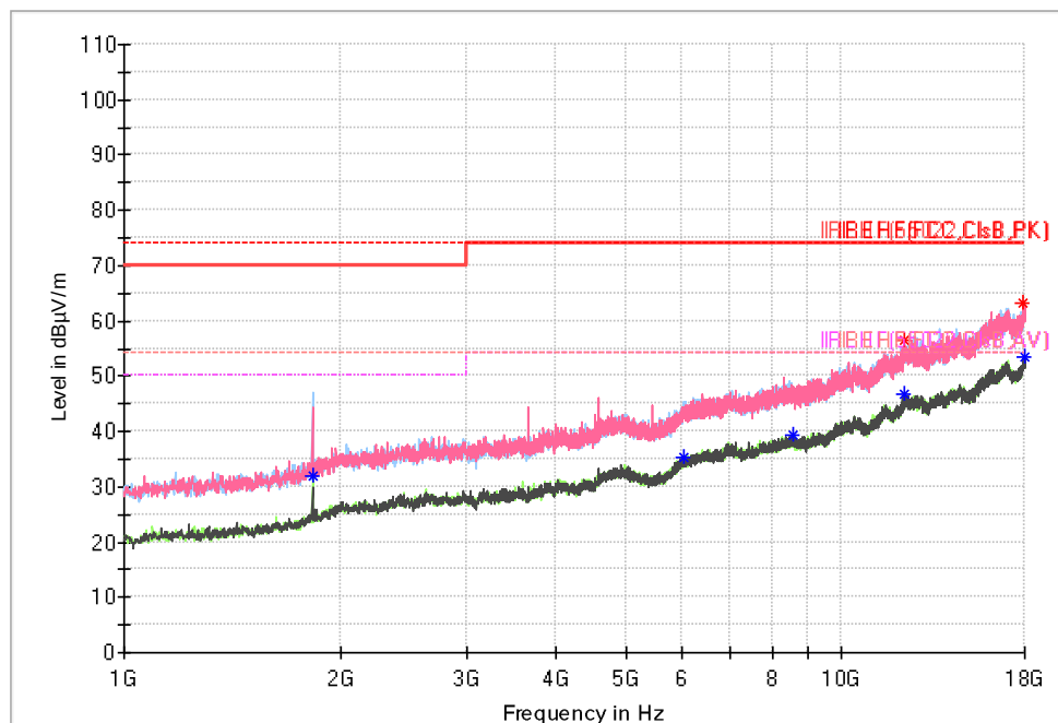
TX Mode (Low Channel)- Radiated Emissions: 1GHz-18GHz
