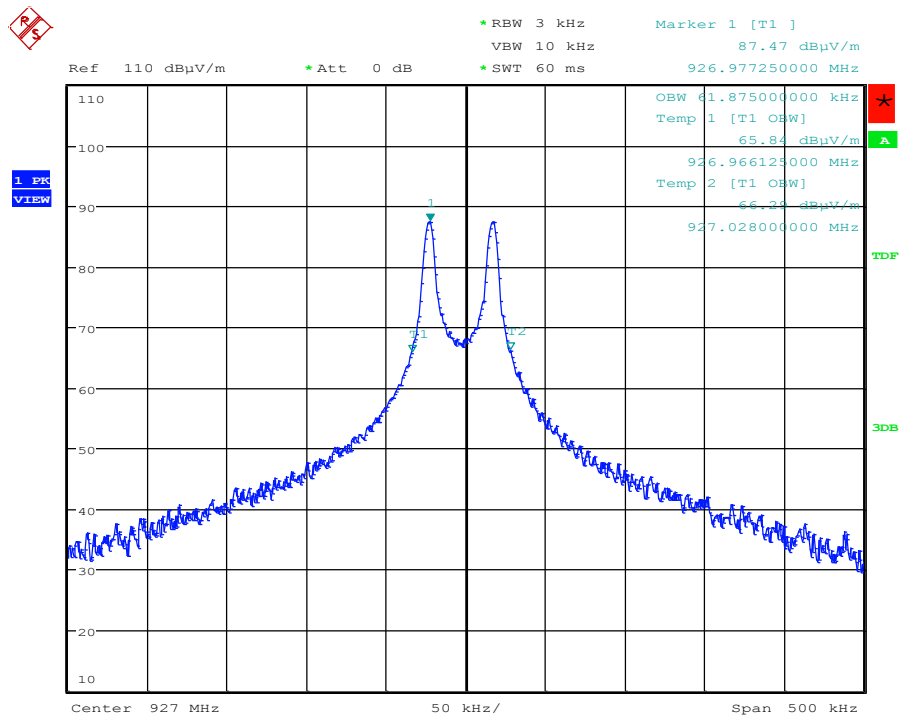
Plot: 99% Occupied Bandwidth of High Channel
