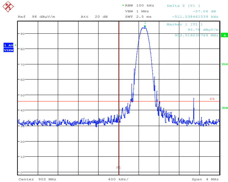
Band edge, low side
