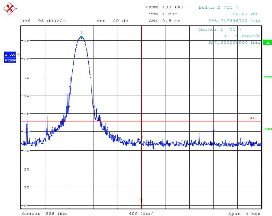
Band edge, high side
