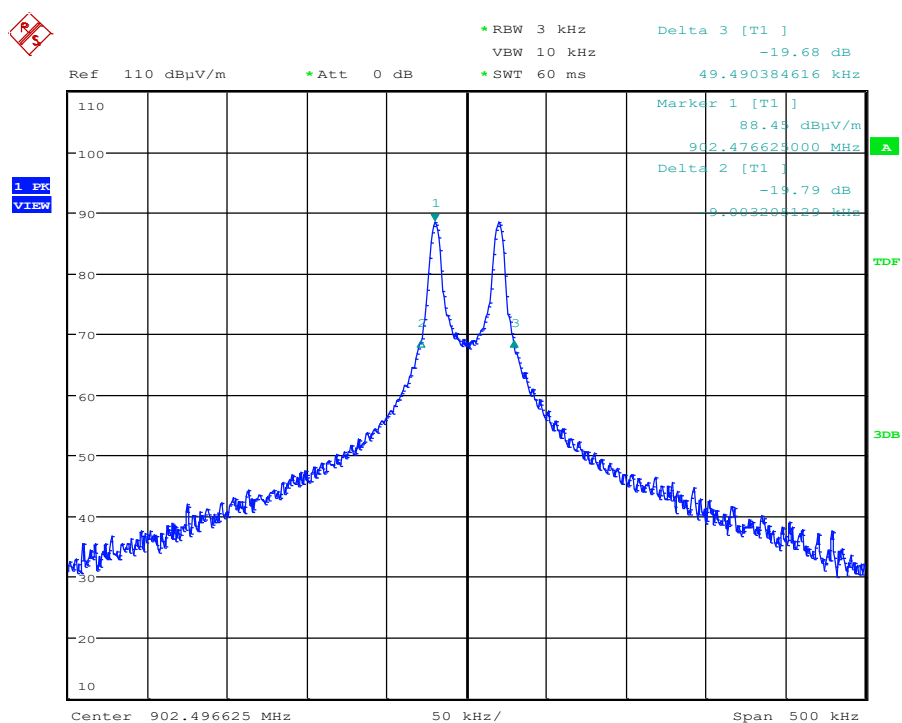
Plot: 20dB Occupied Bandwidth of Low Channel
