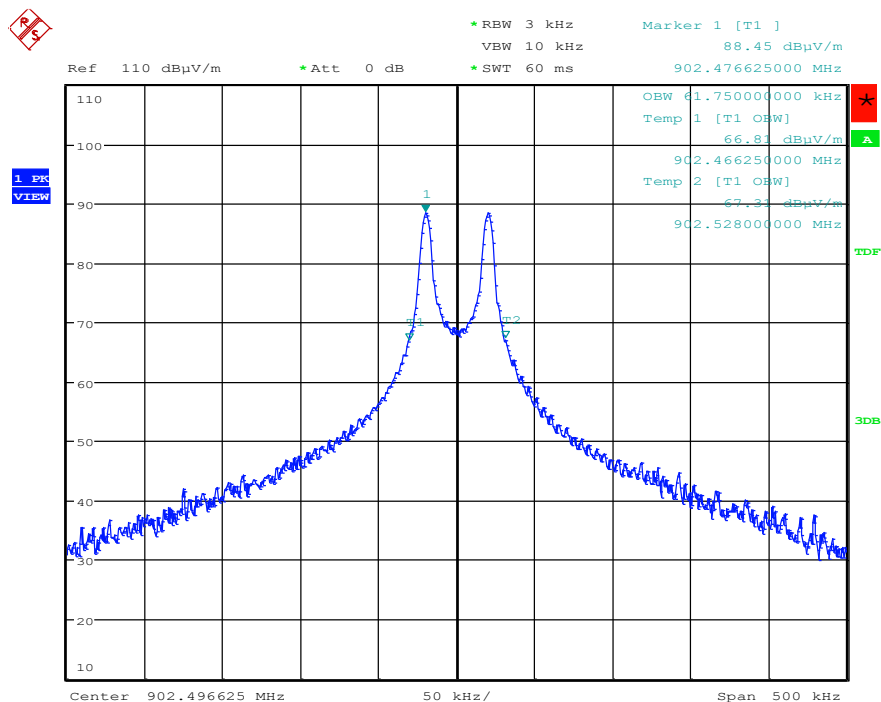
Plot: 99% Occupied Bandwidth of Low Channel
