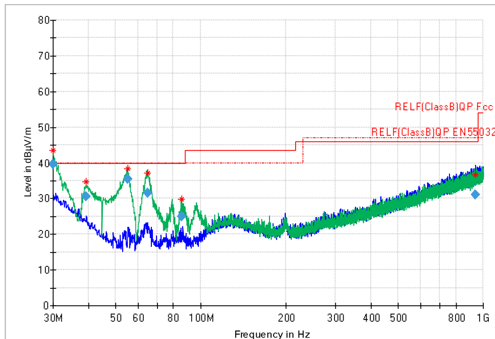
Unintentional Radiated Emissions: 30-1000MHz
