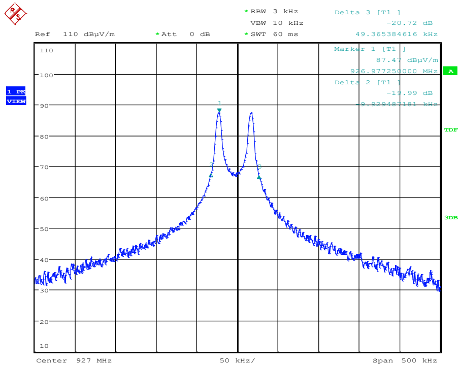
Plot: 20dB Occupied Bandwidth of High Channel
