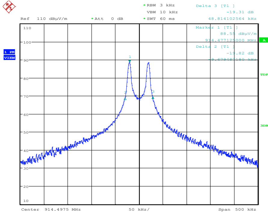
Plot: 20dB Occupied Bandwidth of Mid Channel
