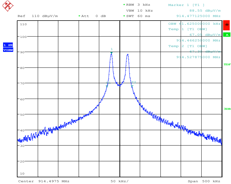
Plot: 99% Occupied Bandwidth of Mid Channel
