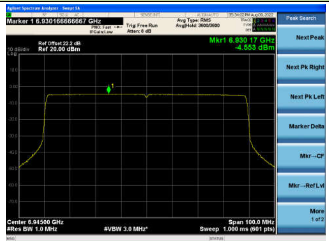
Channel 199 (6945MHz)
