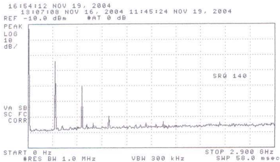
Figure 6.2. Emission spectrum of the DUT (CW). The amplitudes are only indicative (not calibrated).
