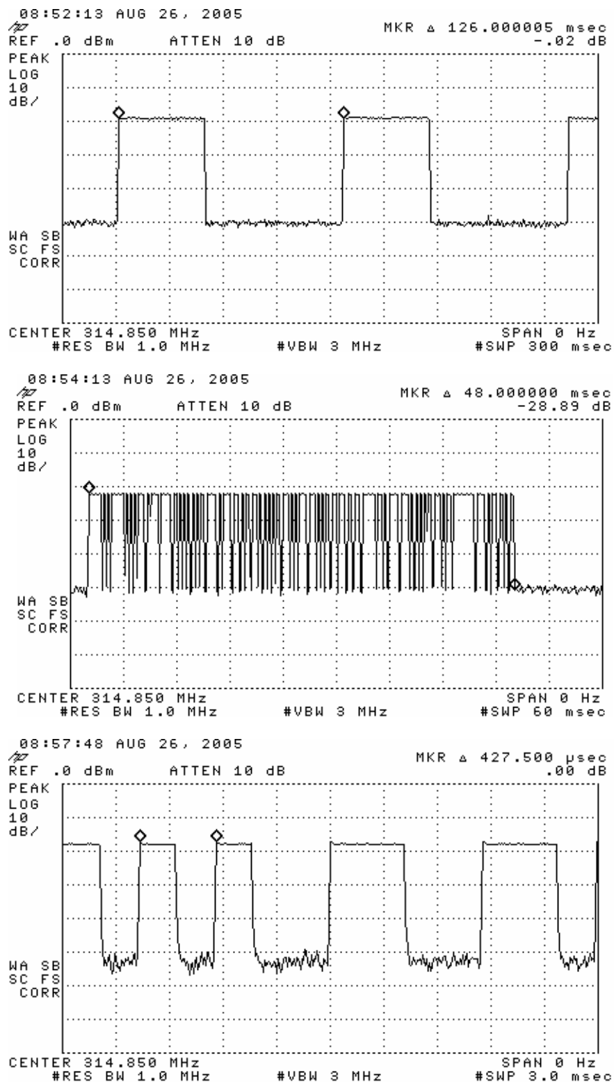
Figure 6.1. Transmissions modulation characteristics: (top) complete transmission, (center) expanded word, (bottom) Manchester encoding.
