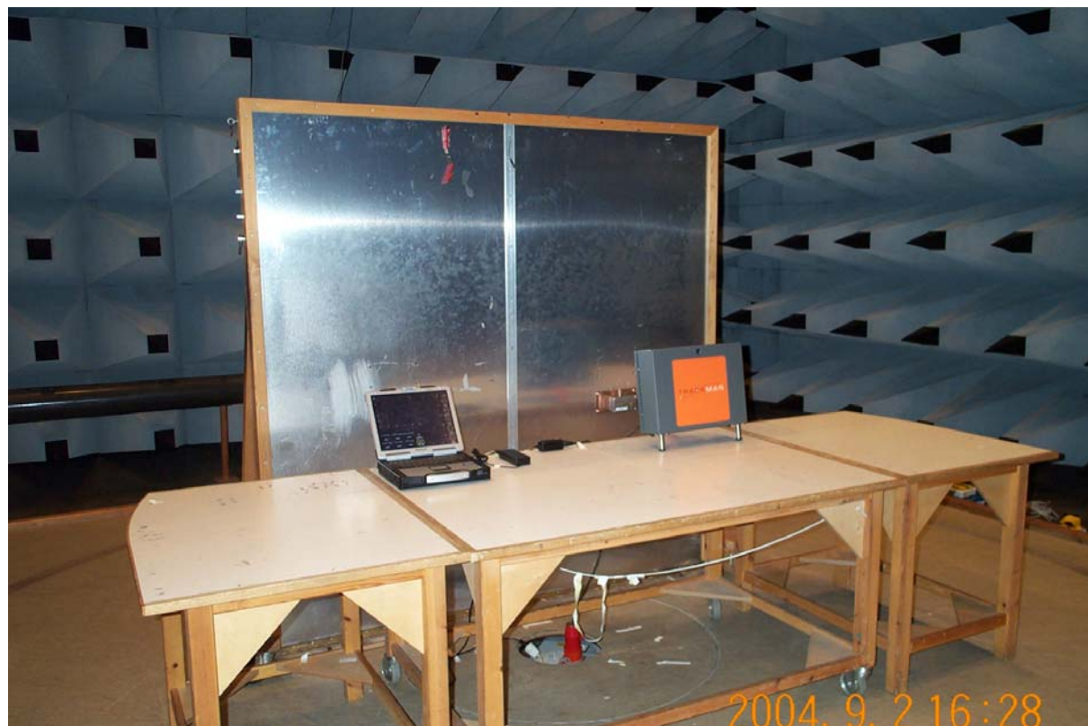
Photo A2.1 Conducted emission 0.15 - 30 MHz.
