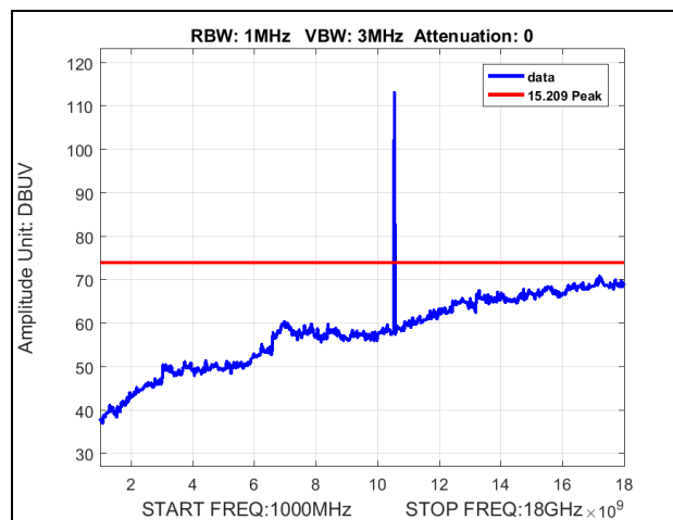
Plot 10. Spurious Emissions, High Channel, 1-18GHz, Peak
