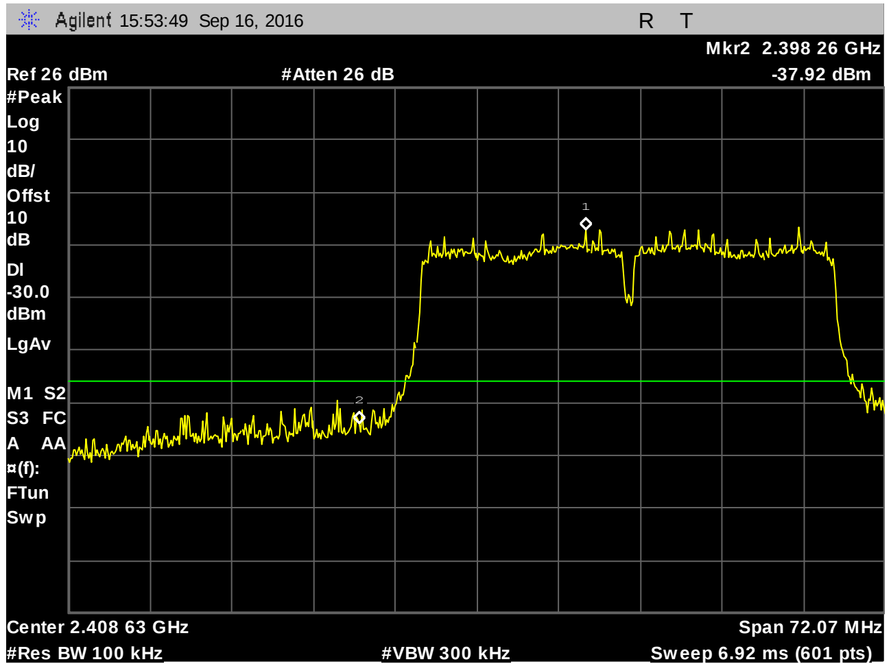
Plot 172. Conducted Band Edge, Ch. 2412, 40MHz, n mode, 30 dBc, Port 1
