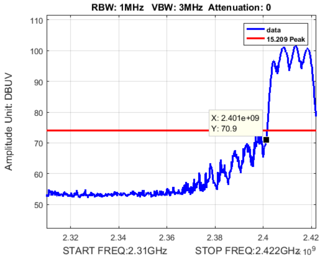
Plot 128. Peak Band Edge Spurious, Bandwidth 20M, Ch. 2412M, g mode
