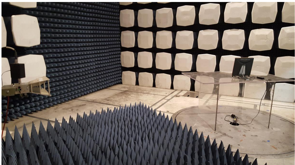
Photograph 4. Radiated Spurious Emissions, Test Setup, Above 1GHz
