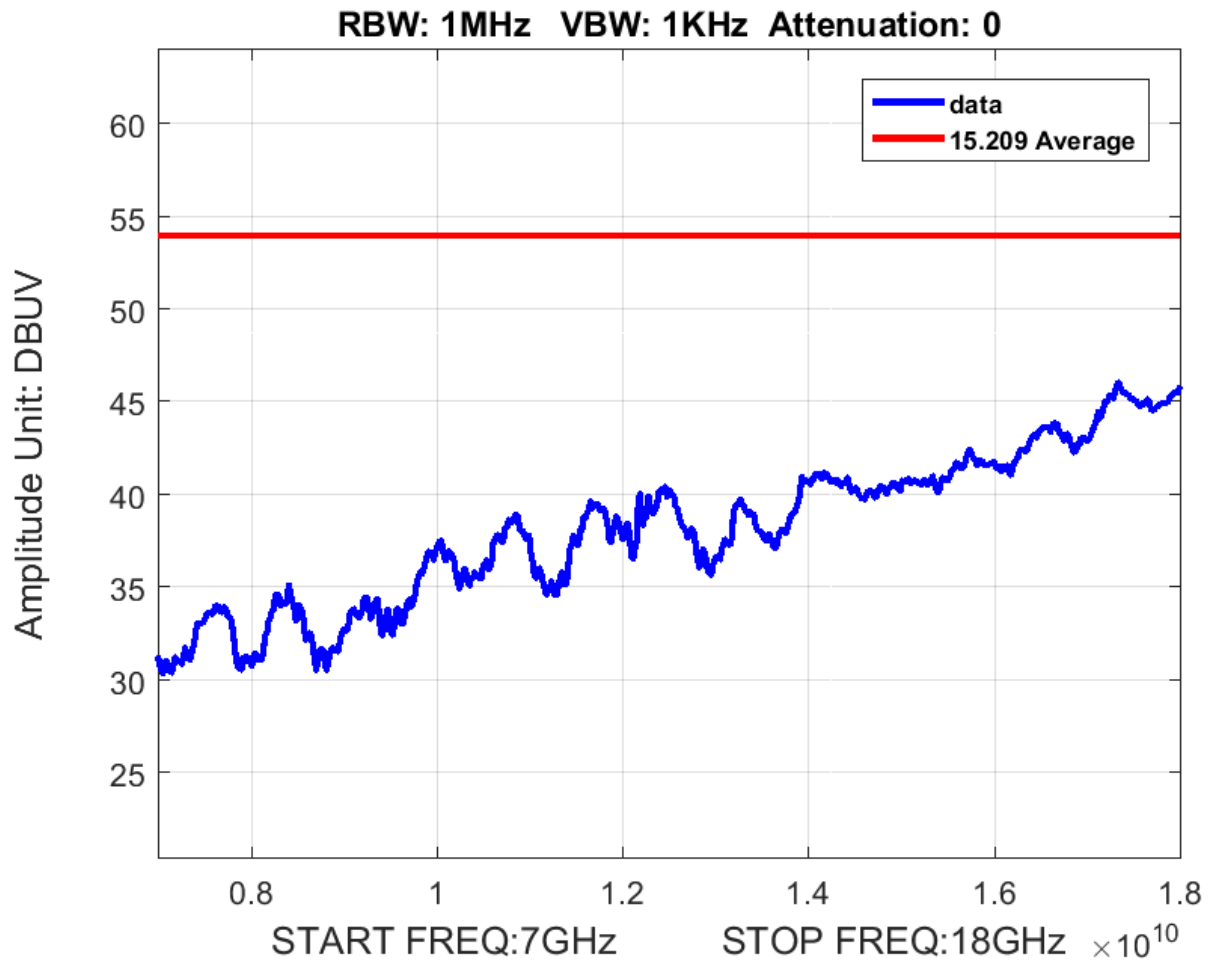
Plot 118. Average Spurious Emission 7-18GHz, Bandwidth 20M, Ch. 2422M, n mode
