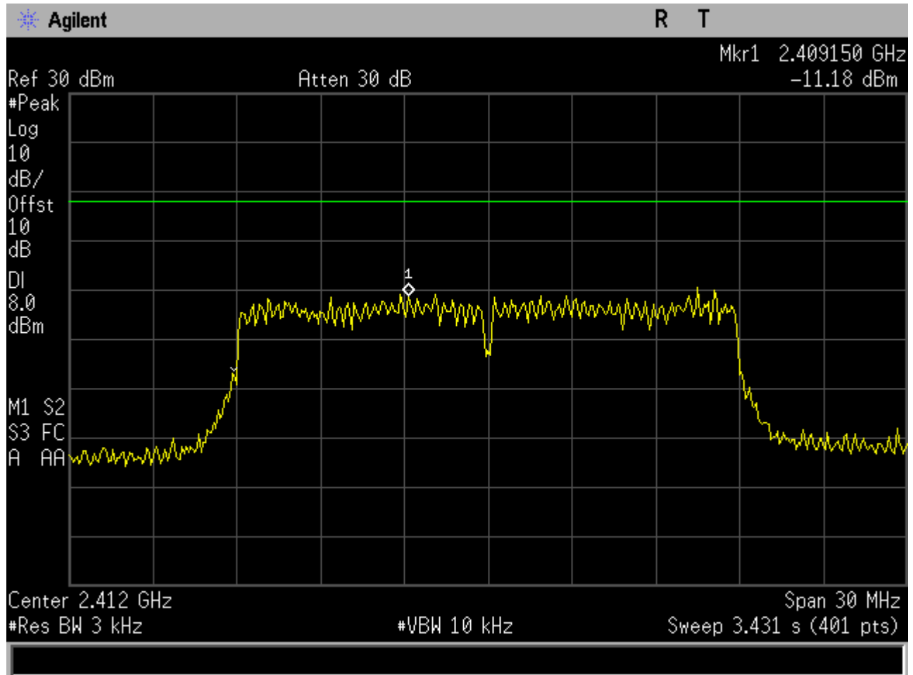
Plot 188. Power Spectral Density, Bandwidth 20M, Ch. 2412M, n mode, Port 2
