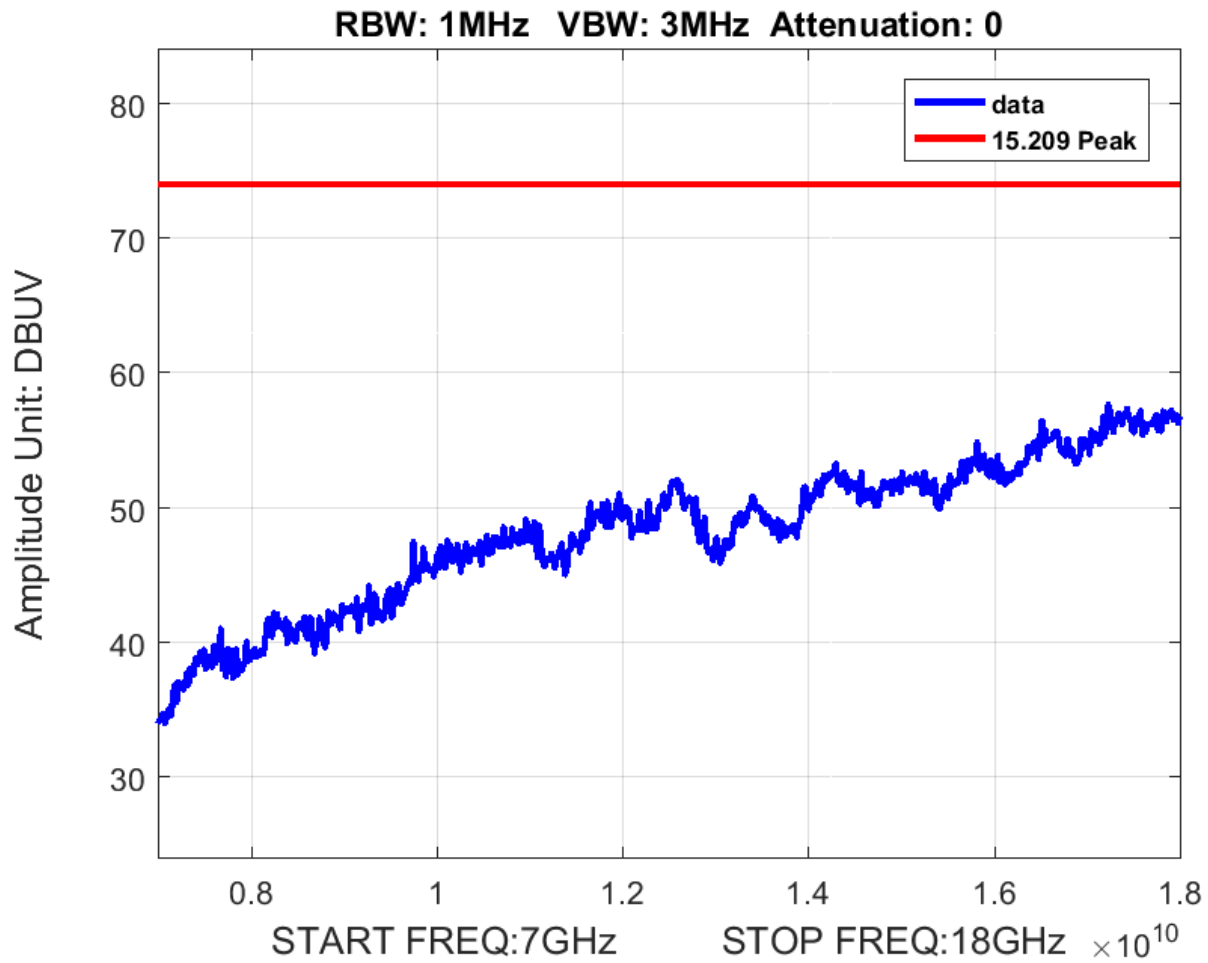
Plot 86. Peak Spurious Emission 7-18GHz, Bandwidth 20M, Ch. 2437M, b mode
