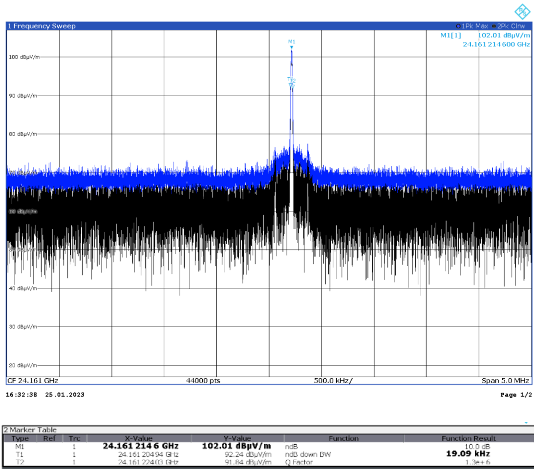
Figure 8.1-2: Occupied bandwidth results (10 dB) high frequency plot
