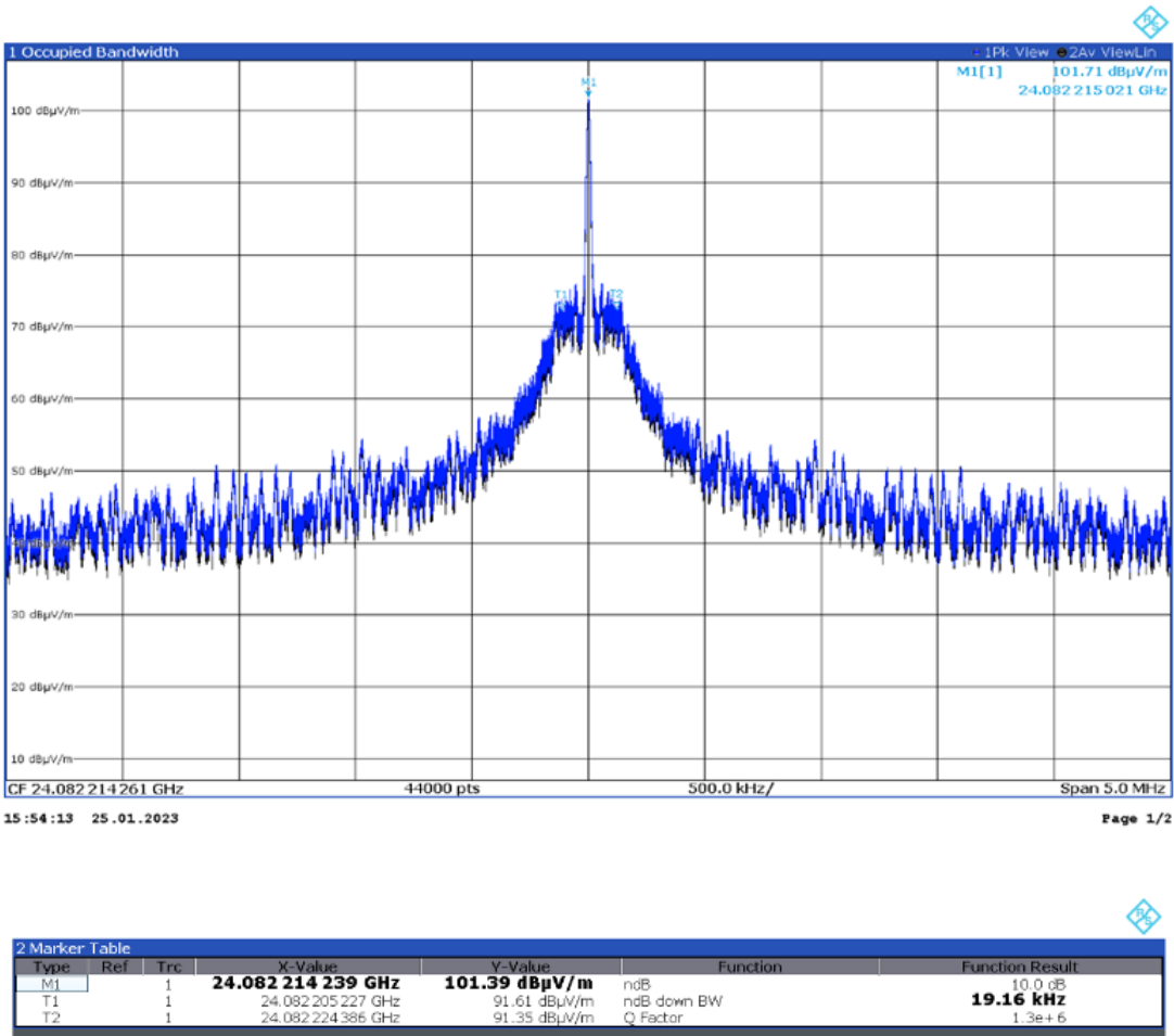
Figure 8.1-1: Occupied bandwidth results (10 dB) low frequency plot
