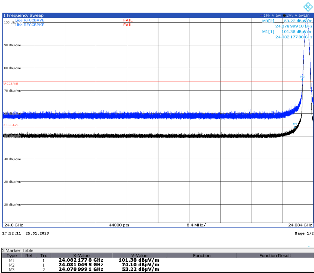
Figure 8.4-1: Band Edges plot – Low edge
