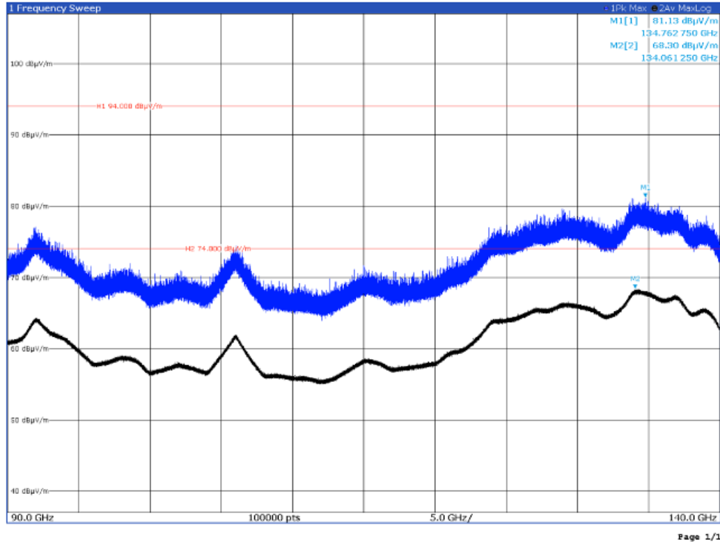
Figure 8.4-9: Radiated emissions plot – Field strength measured from 90 to 140 GHz, Rx antenna in horizontal and vertical polarization, respectively
