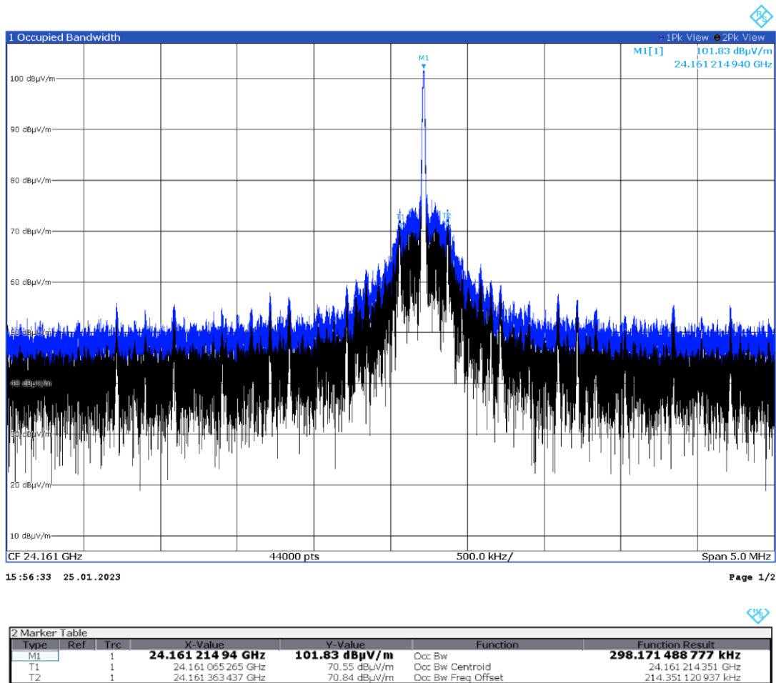
Figure 8.2-2: Occupied bandwidth results (99%) high frequency plot
