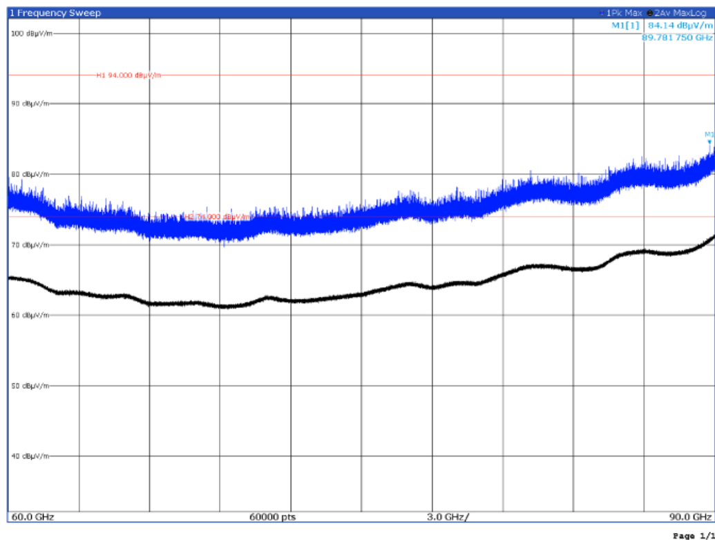
Figure 8.4-8: Radiated emissions plot – Field strength measured from 60 to 90 GHz, Rx antenna in horizontal and vertical polarization, respectively.
