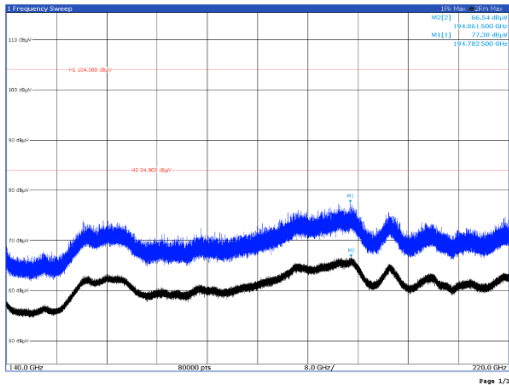
Figure 8.4-10: Radiated emissions plot – Field strength measured from 140 to 220 GHz, Rx antenna in horizontal and vertical polarization, respectively.
