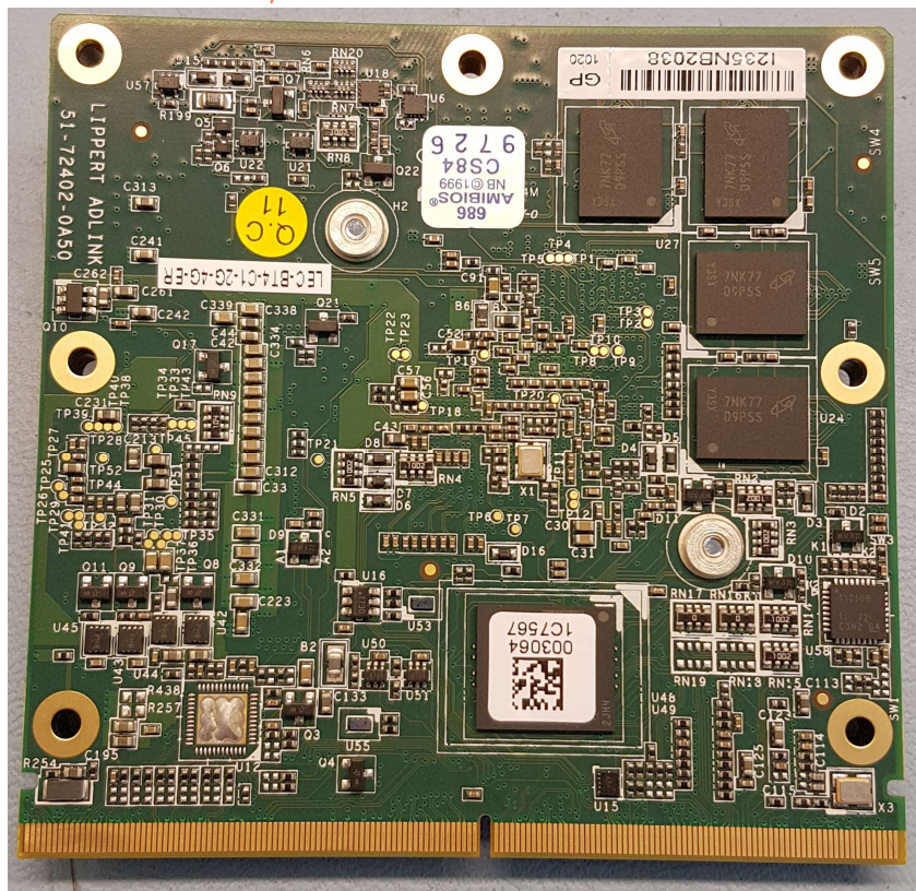
TMB4A CPU module – EU050009, seen from the back:
