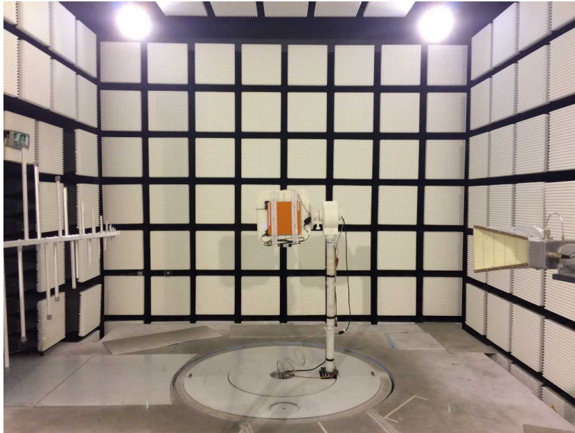
Photo 5: RSE test setup >1GHz
