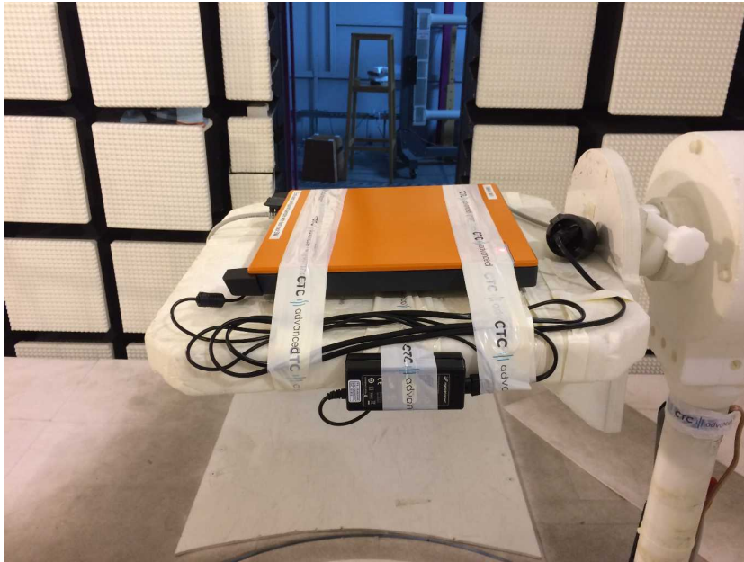
Photo 3: RSE test setup >1GHz
