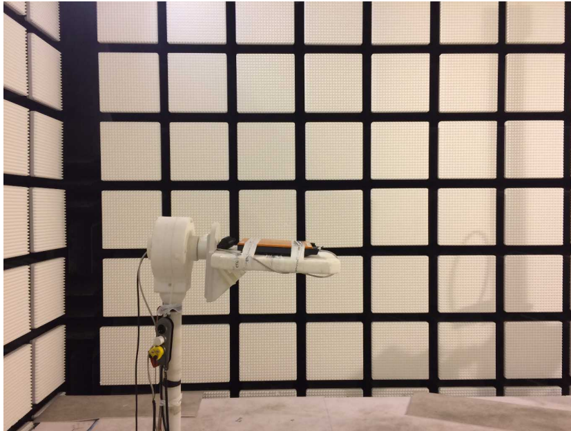
Photo 1: RSE test setup >1GHz
