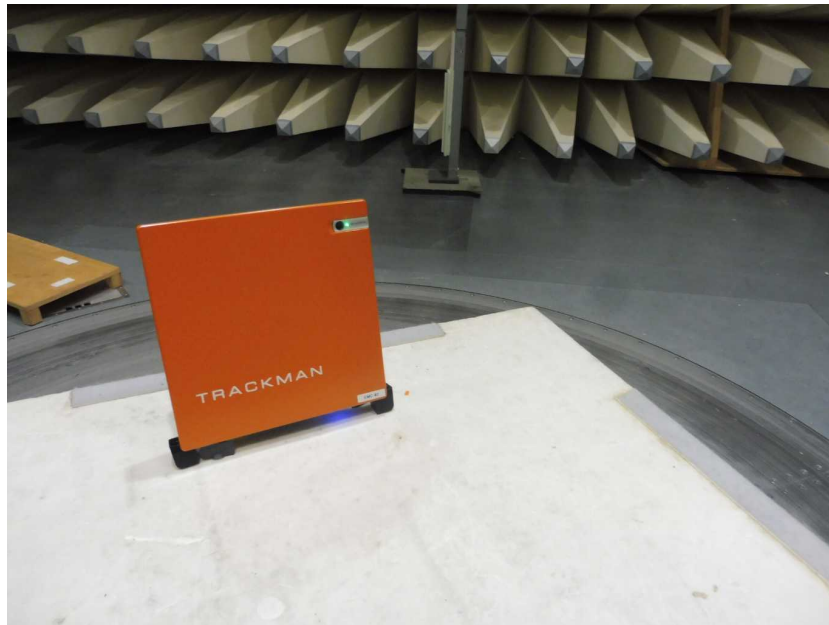
Photo 9: RSE test setup <1GHz
