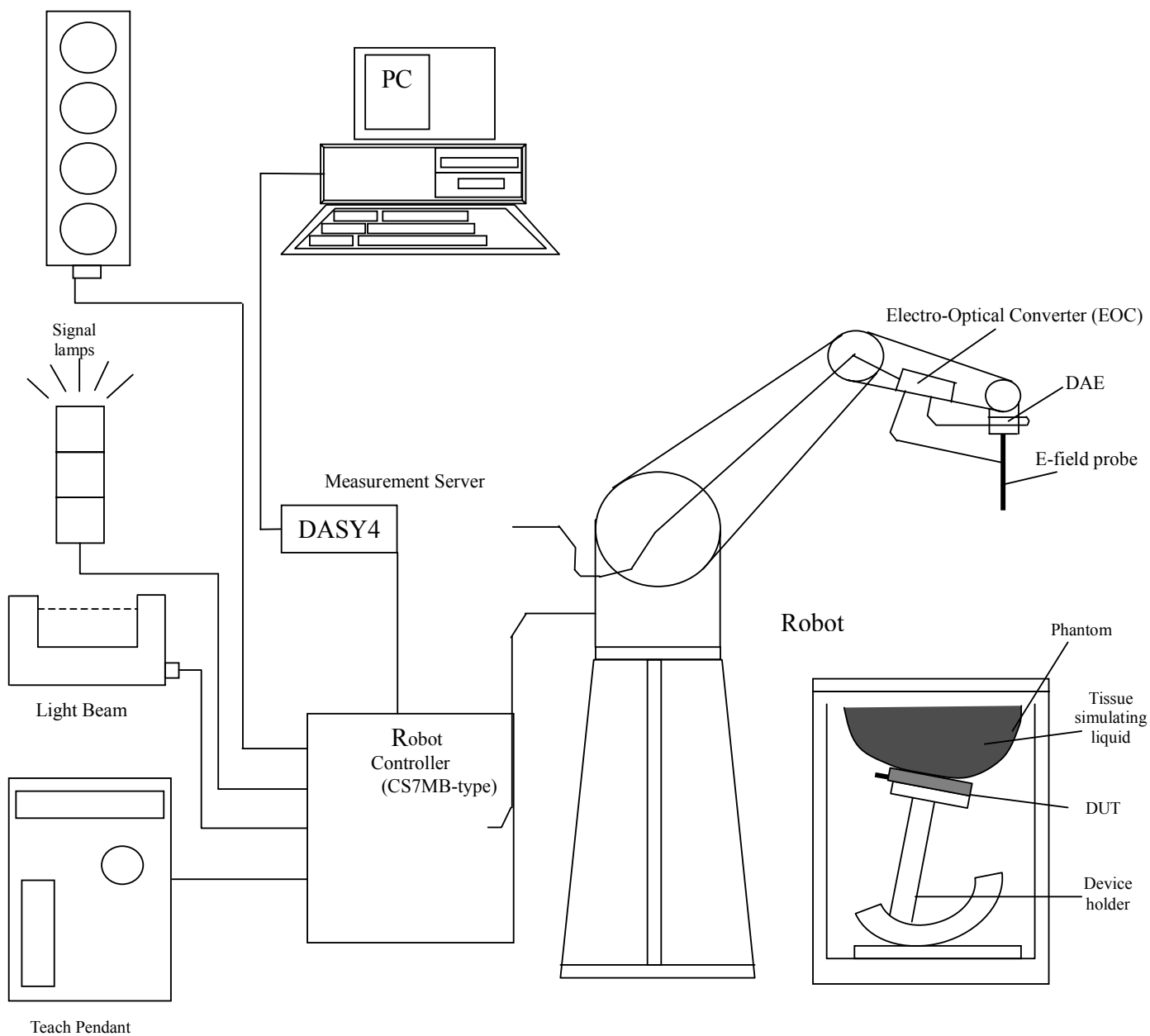
Fig. 5.1 DASY4 system
