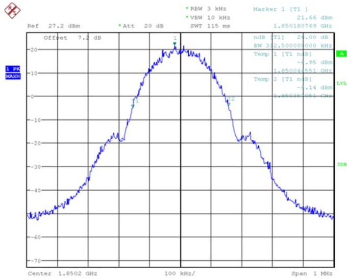
Channel 512- Emission Bandwidth (-26dBc BW)
