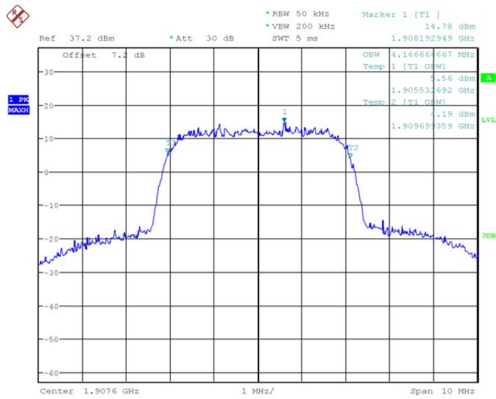
Channel 9538-Occupied Bandwidth
