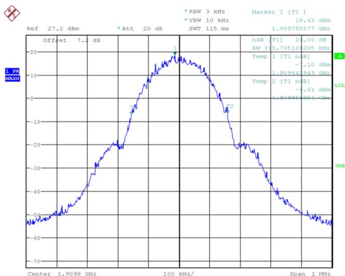
Channel 810- Emission Bandwidth (-26dBc BW)
