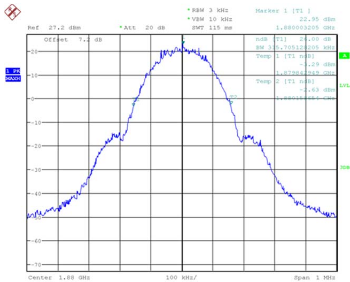
Channel 661- Emission Bandwidth (-26dBc BW)
