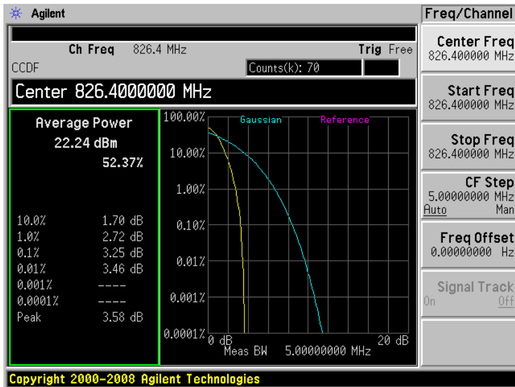
WCDMA Band V CH4132
