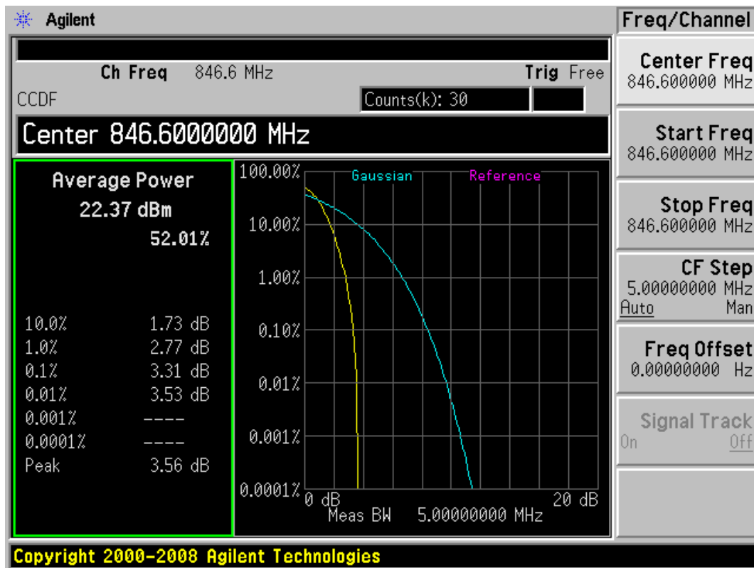
WCDMA Band V CH4233
