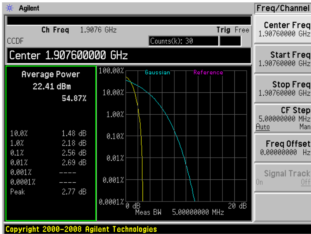
WCDMA Band II CH9538
