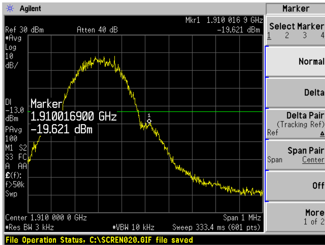
GSM1900 810 Channel
