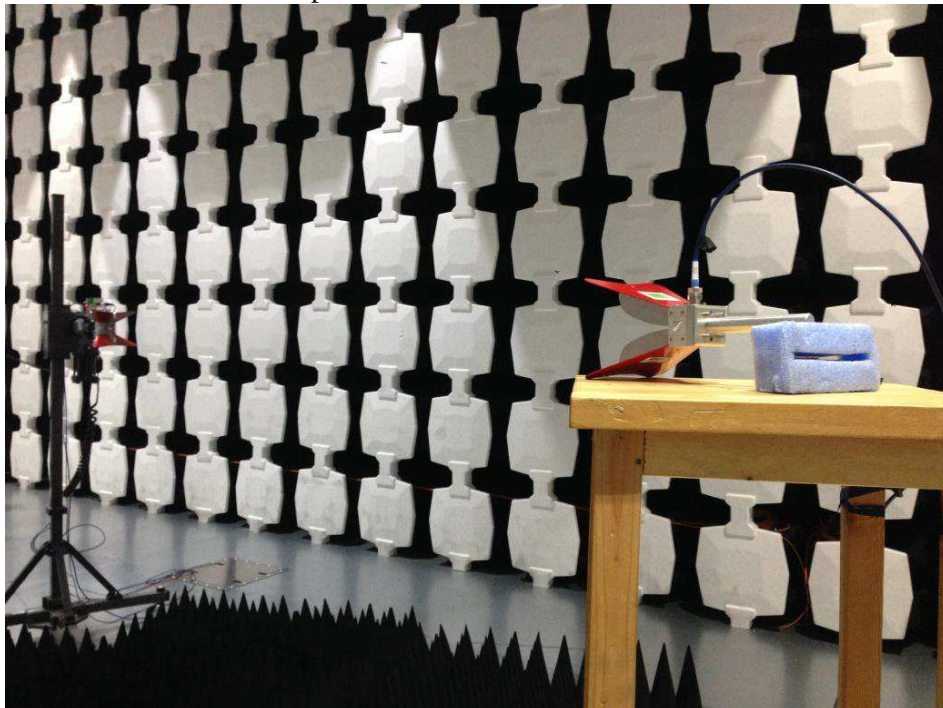
Step 2: Substitution Antenna test
