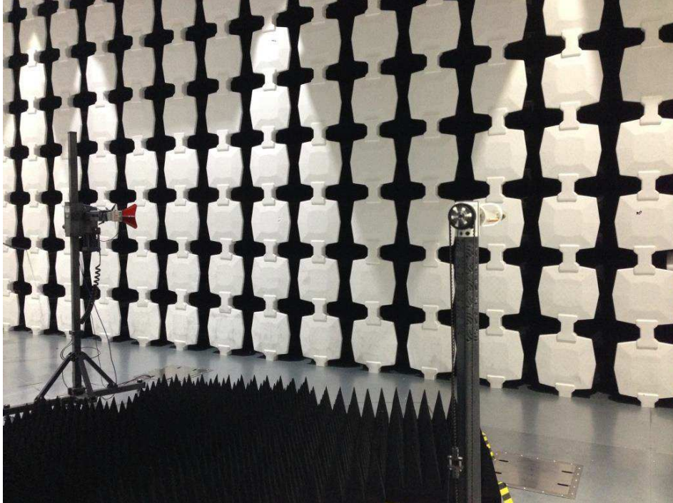
Step 1: EUT Radiated emission test
