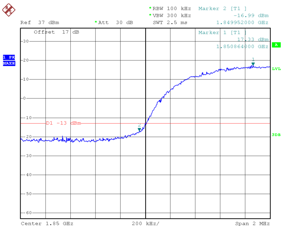
(Plot K: WCDMA 1900 Channel = 9262)
