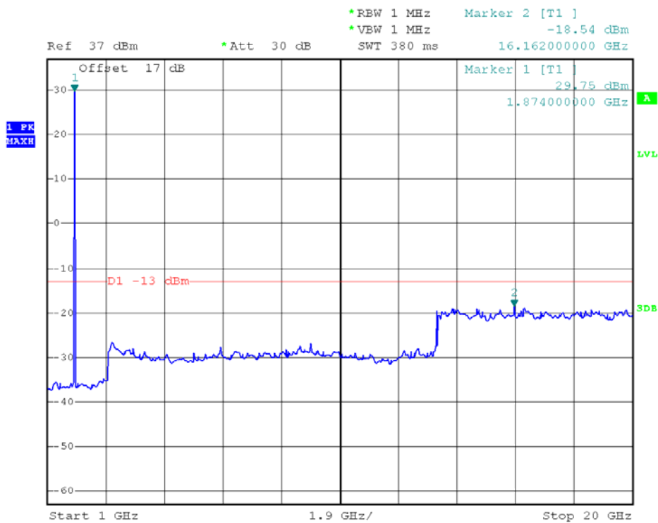
EDGE 1900MHz Channel = 661, 1GHz to 20GHz
