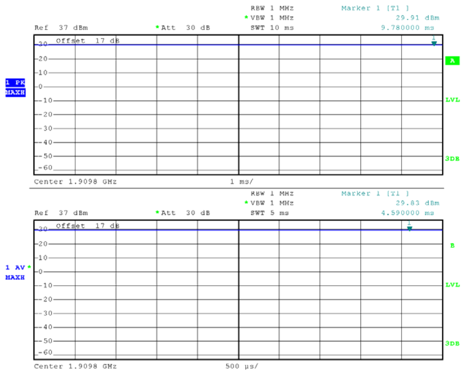
(Plot A3: GSM 1900MHz Channel = 810)
