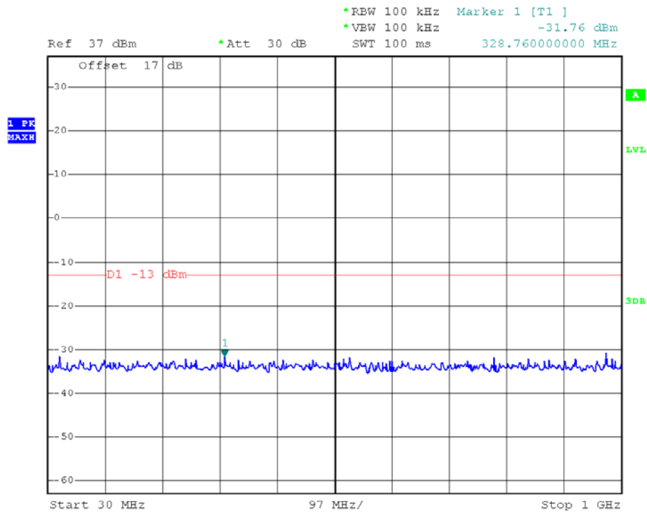
EDGE 1900MHz Channel = 661, 30MHz to 1GHz
