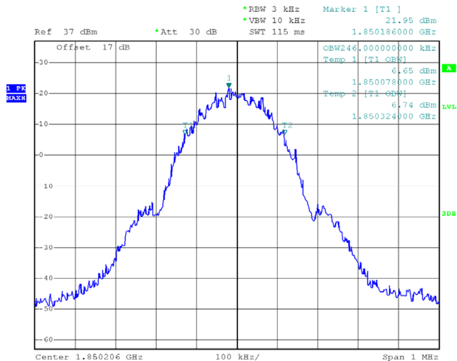
(Plot B2: GSM 1900MHz Channel = 512 99% Occupied Bandwidth)
