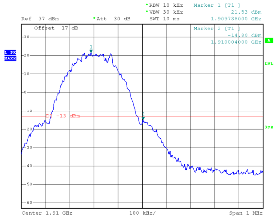
(Plot D: GSM 1900 Channel = 810)
