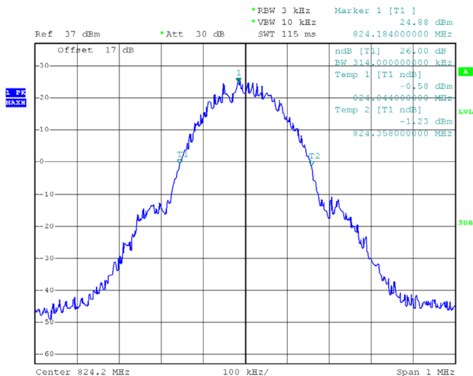
(Plot C1: EDGE 850MHz Channel = 128 26dB bandwidth)
