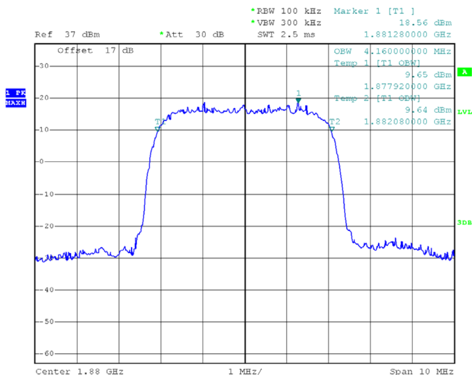
(Plot F4: WCDMA 1900MHz Channel = 9400 99% Occupied Bandwidth)
