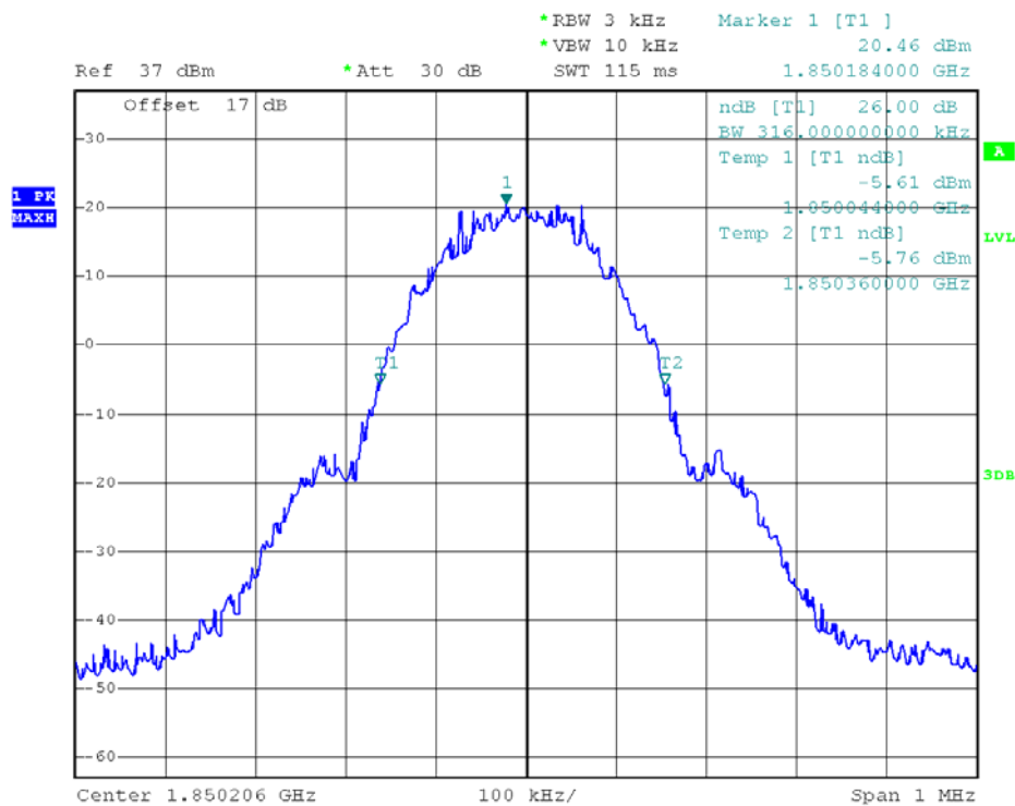
(Plot B1: GSM 1900MHz Channel = 512 26dB bandwidth)
