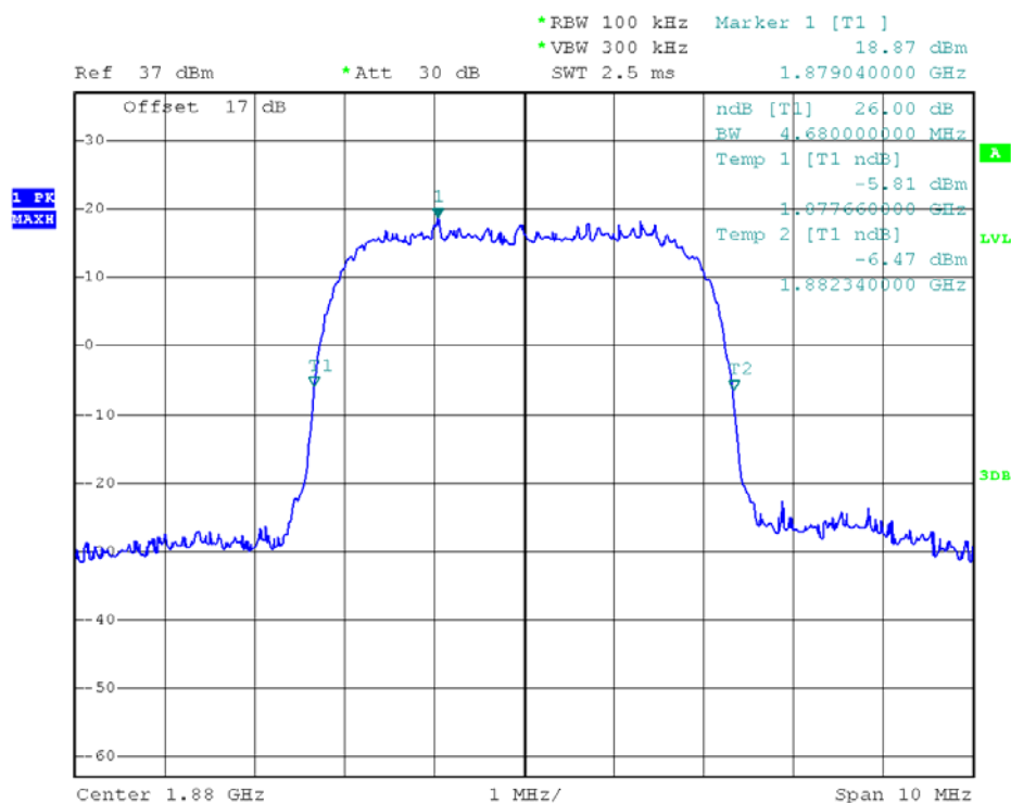
(Plot F3: WCDMA 1900MHz Channel = 9400 26dB bandwidth)
