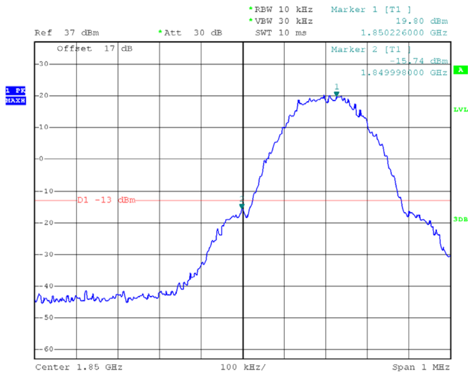
(Plot G: EDGE 1900 Channel = 512)
