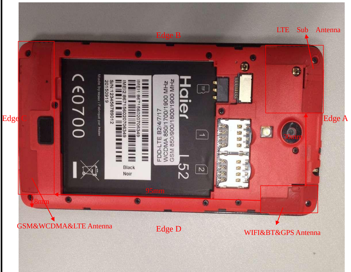
Fig. 3 Position of the antennas
