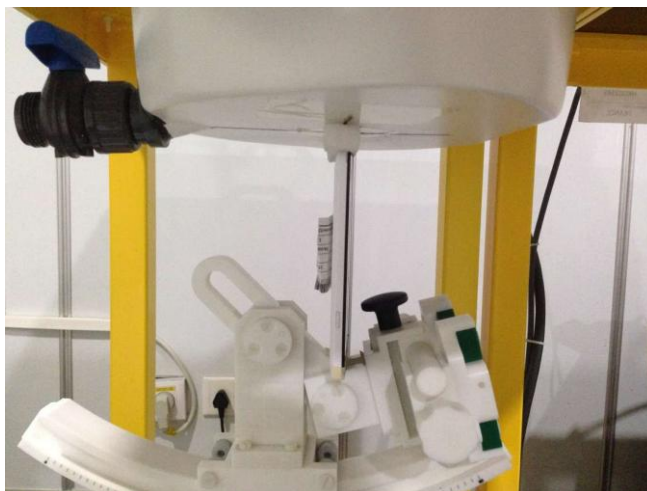
Fig.10 Body Edge C(UP,10mm separation)
