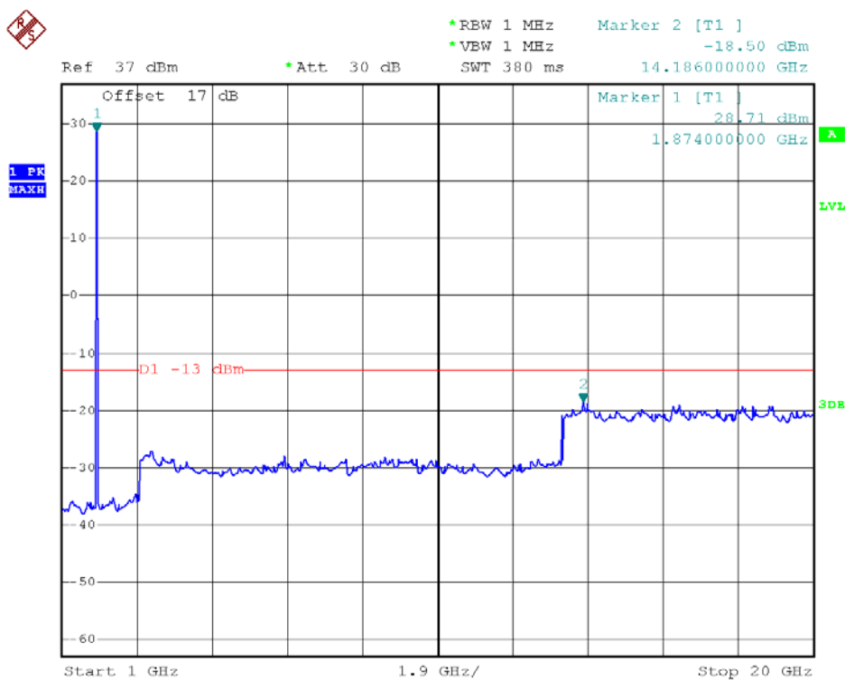
EDGE 1900MHz Channel = 661, 1GHz to 20GHz
