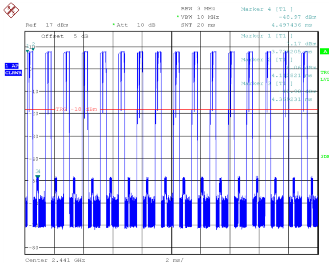
Fig.64 Time of occupancy (Dwell Time): Ch39,Packet 2-DH1
