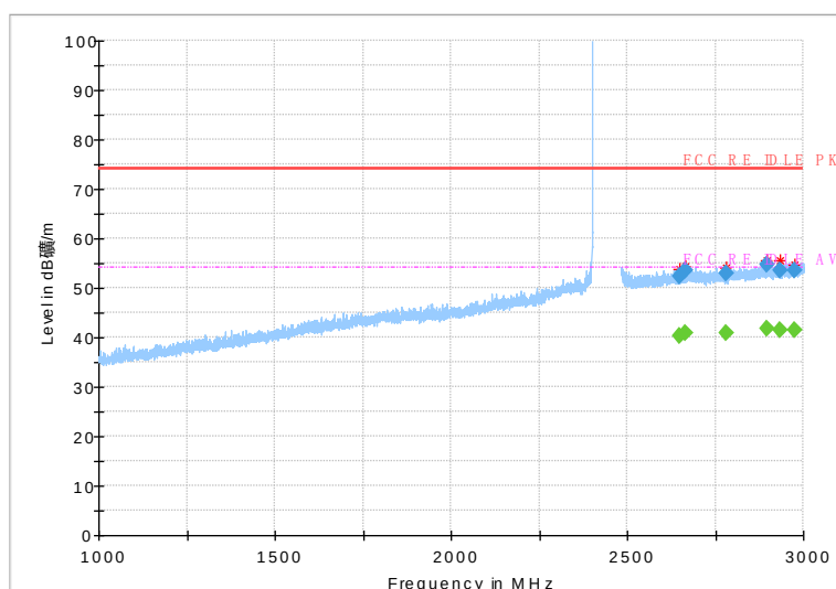
Fig.47 Radiated emission: \pi/4 DQPSK, Ch0, 1GHz~3GHz
