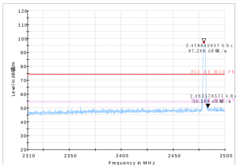
Fig.56 Radiated emission (Power): 8DPSK, high channel
