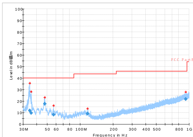
Fig.46 Radiated emission: \pi/4 DQPSK, Ch0, 30MHz~1GHz
