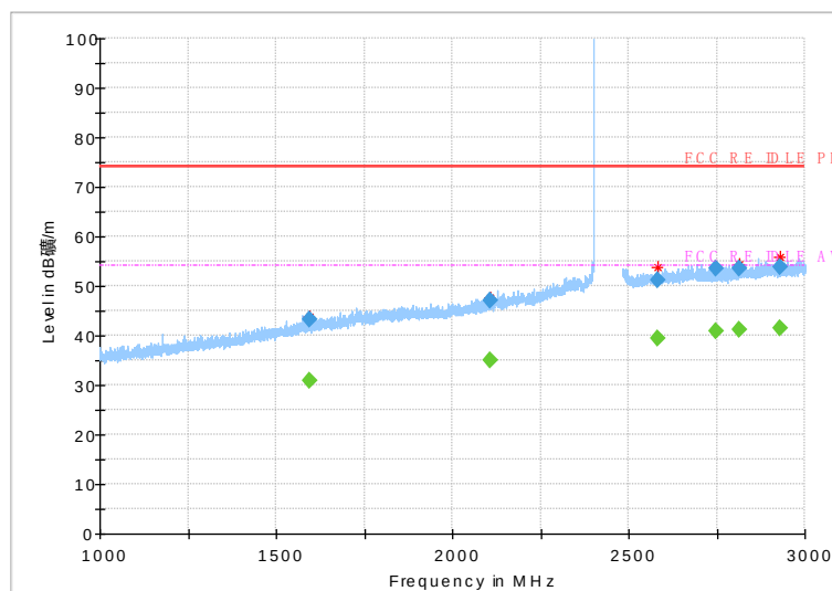
Fig.41 Radiated emission: GFSK, Ch0, 1GHz~3GHz
