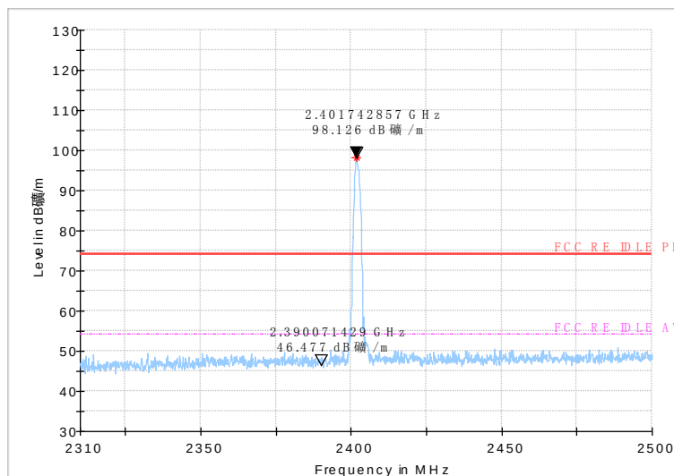
Fig.55 Radiated emission (Power): 8DPSK, low channel
