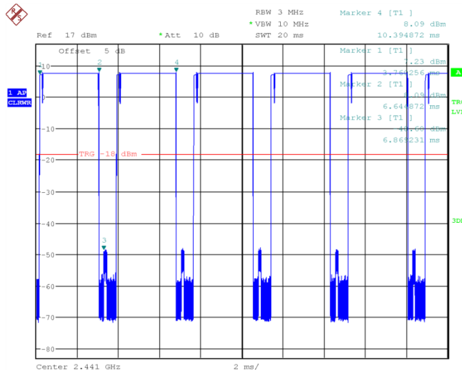
Fig.68 Time of occupancy (Dwell Time): Ch39,Packet 2-DH5
