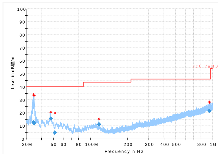
Fig.40 Radiated emission: GFSK, Ch0, 30MHz~1GHz
