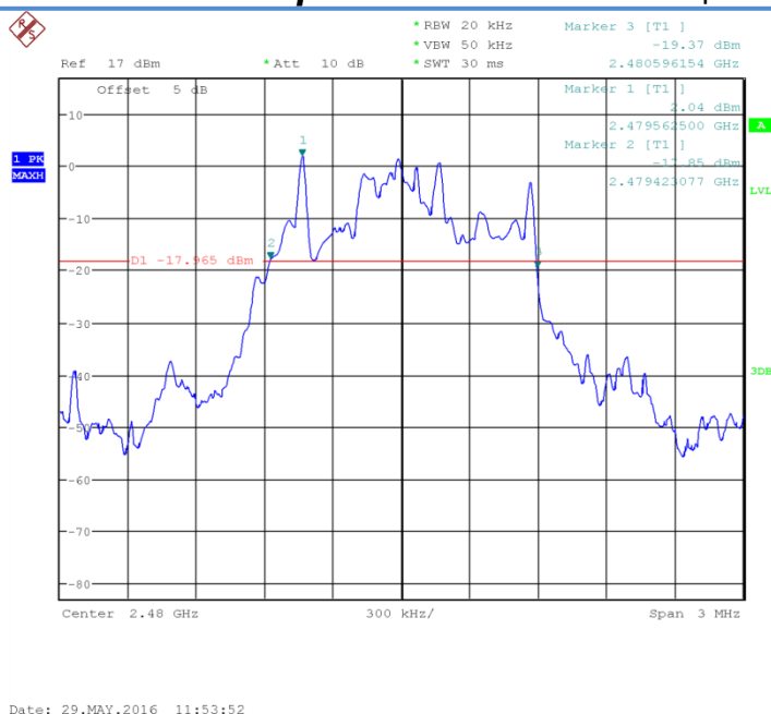
Fig.84 20dB Bandwidth: 8DPSK, Ch78
