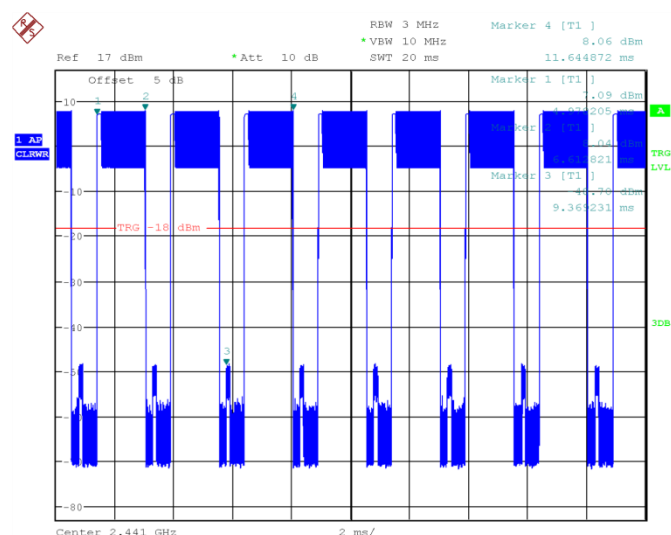
Fig.72 Time of occupancy (Dwell Time): Ch39,Packet 3-DH3
