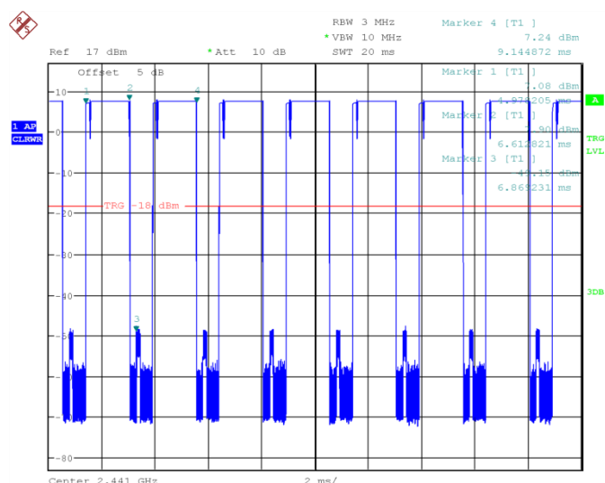
Fig.66 Time of occupancy (Dwell Time): Ch39,Packet 2-DH3
