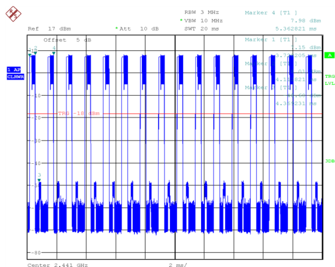
Fig.70 Time of occupancy (Dwell Time): Ch39,Packet 3-DH1
