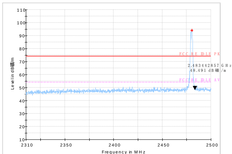
Fig.50 Radiated emission (Power): \pi/4 DQPSK, high channel
