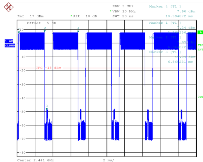
Fig.74 Time of occupancy (Dwell Time): Ch39,Packet 3-DH5
