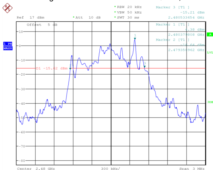
Fig.80 20dB Bandwidth: \pi/4 DQPSK, Ch39
