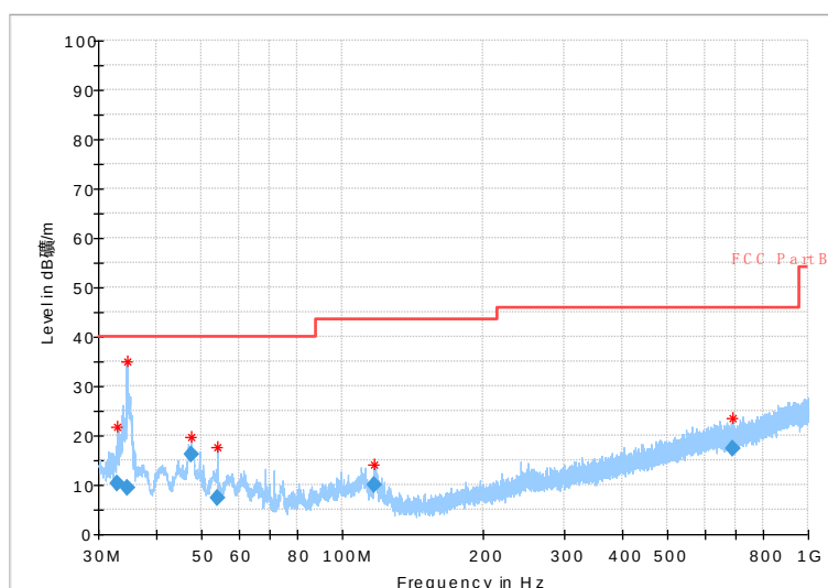
Fig.52 Radiated emission: 8DPSK, Ch0, 30MHz~1GHz
