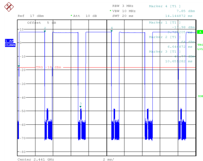
Fig.62 Time of occupancy (Dwell Time): Ch39,Packet DH5
