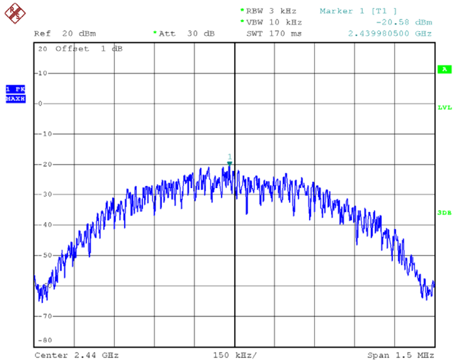
PSD Plot on Channel 19
