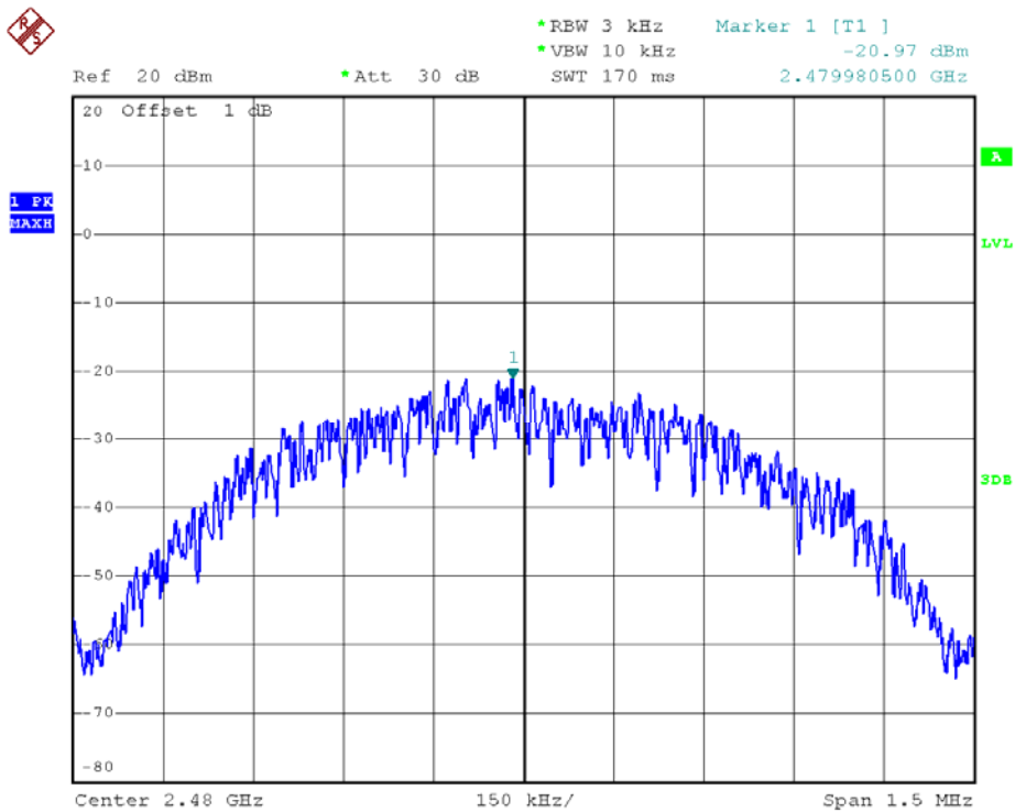
PSD Plot on Channel 39
