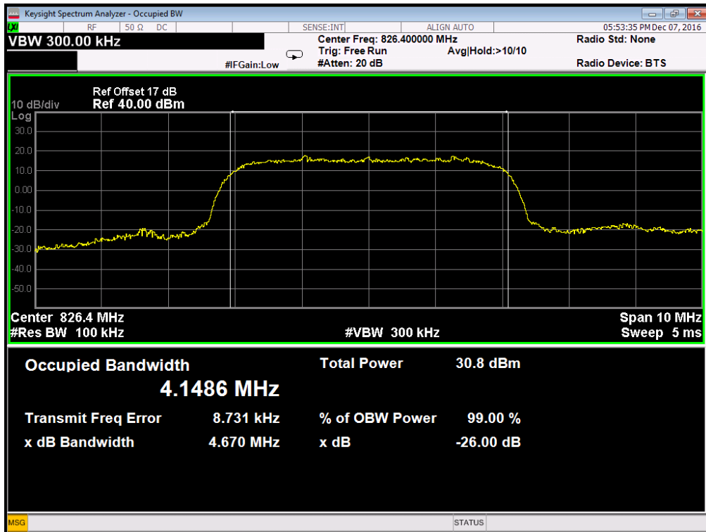
(Plot E1: WCDMA 850MHz Channel = 4132 Occupied bandwidth)
