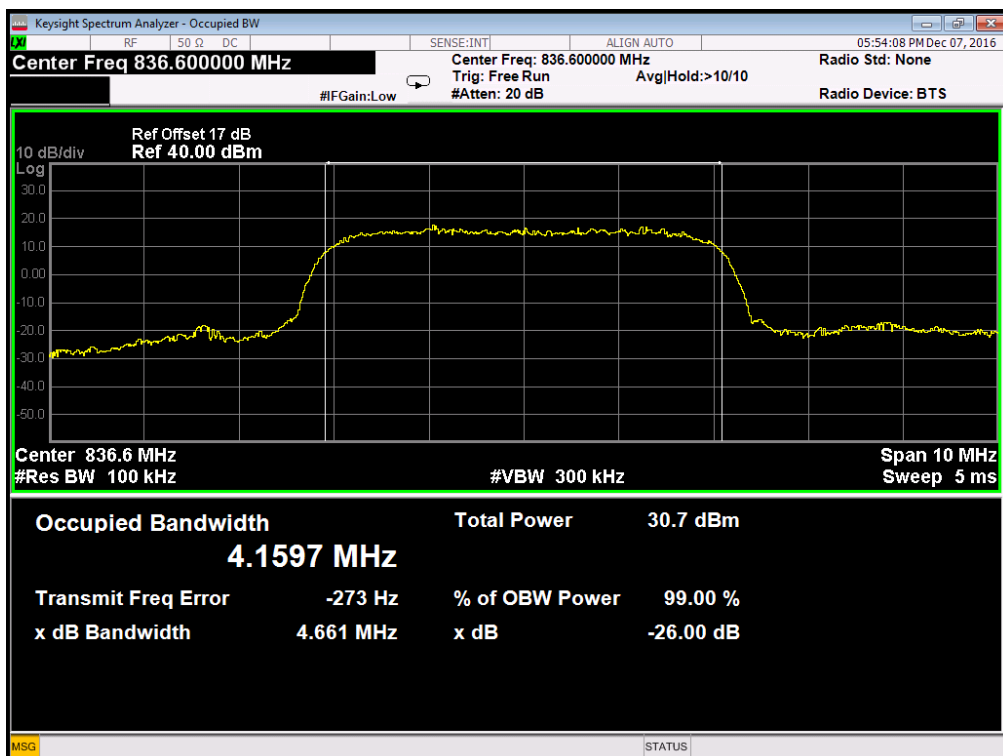
(Plot E2: WCDMA 850MHz Channel = 4183 Occupied bandwidth)
