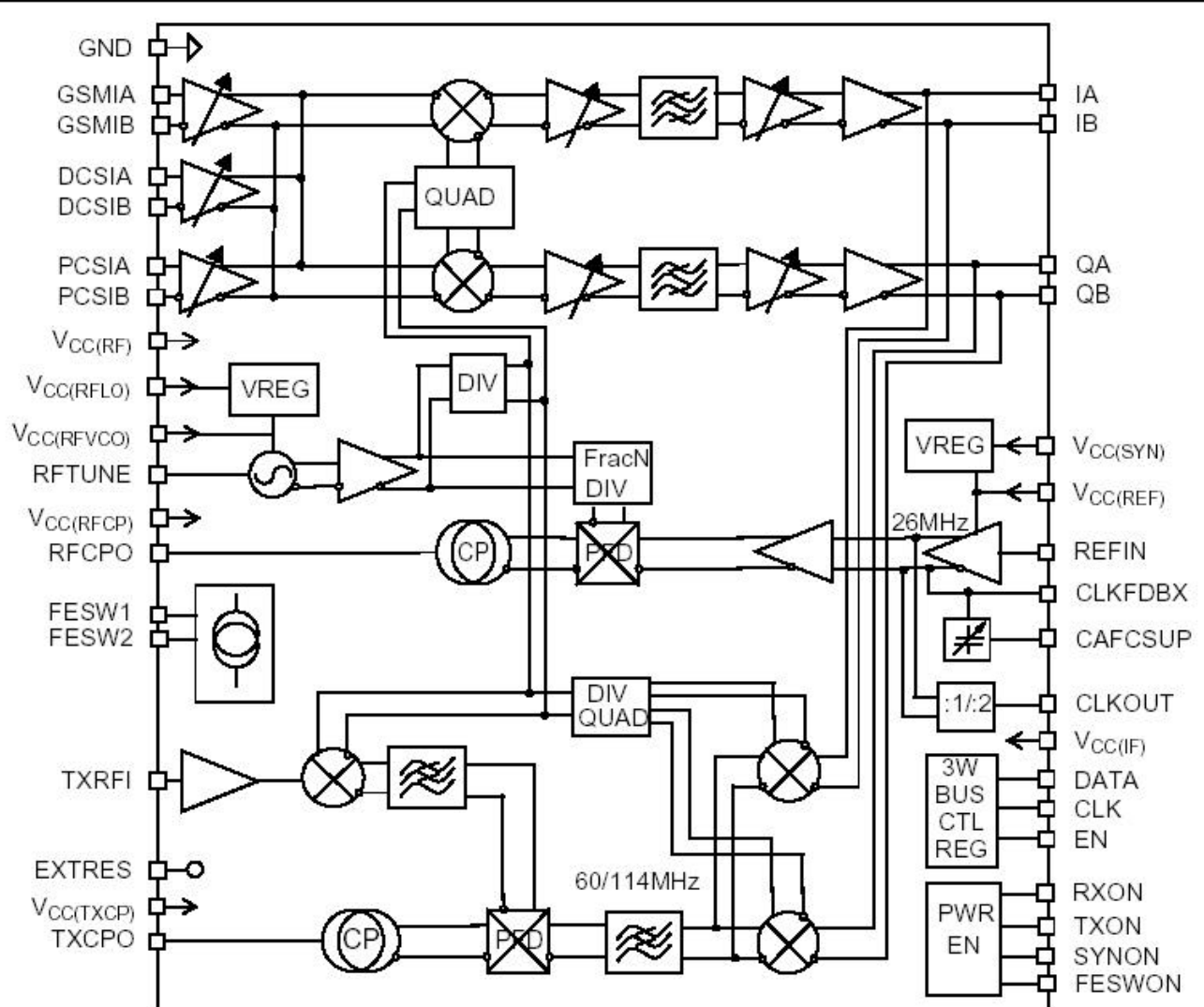
Fig.1 Block diagram.
