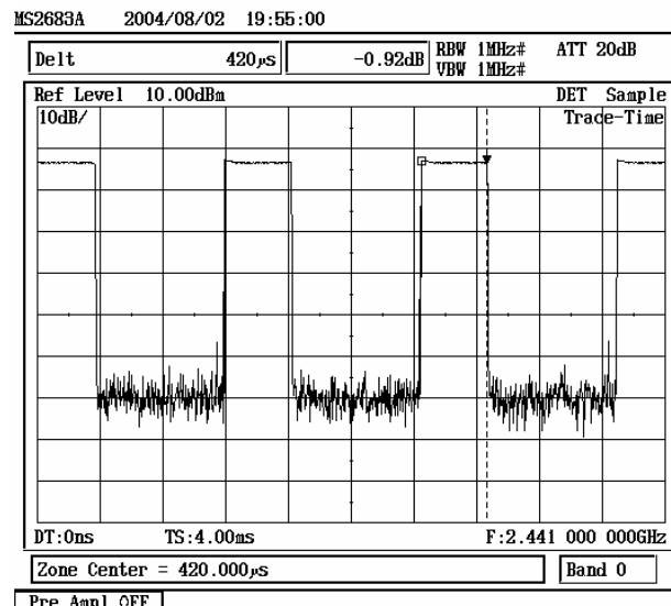
DH1 2441MHz
