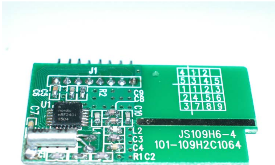
Internal Photo - 3
