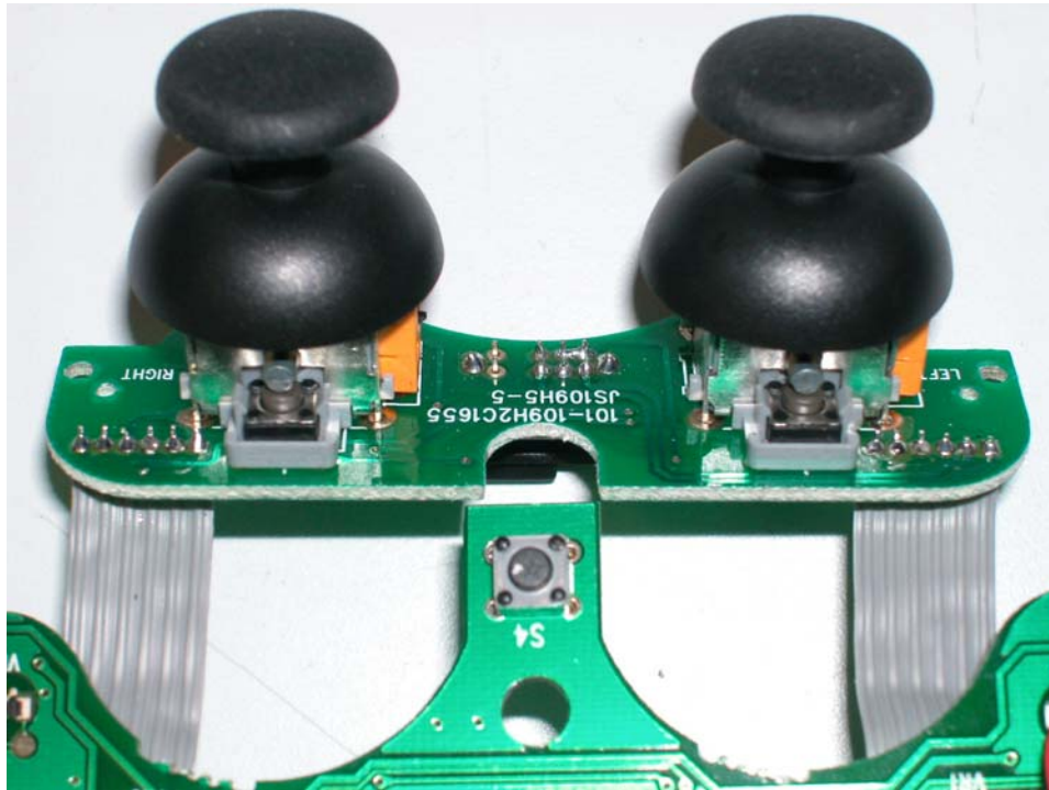
Internal Photo - 11
