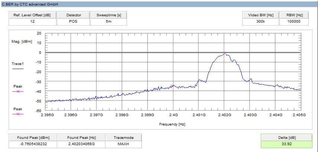
Plot 1: Lower band edge
