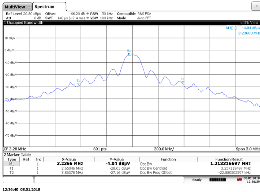
Plot 2: 99 % emission bandwidth, 320 kbit/s
