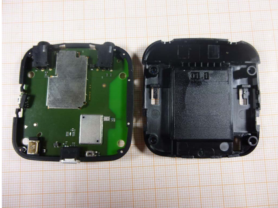
Photo 5: PCB front side view
