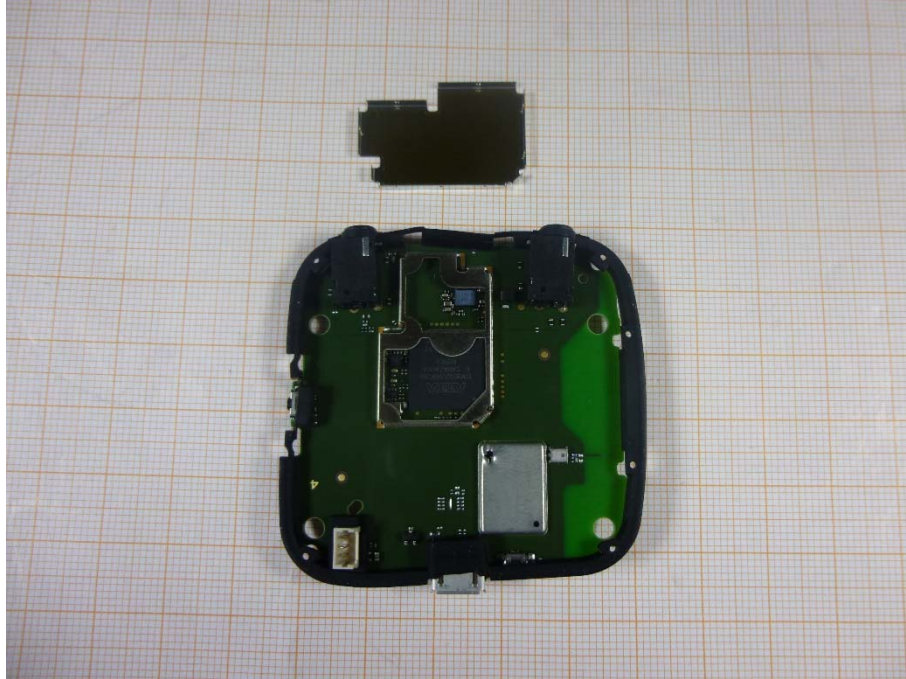
Photo 7: PCB front side view (shielding removed)
