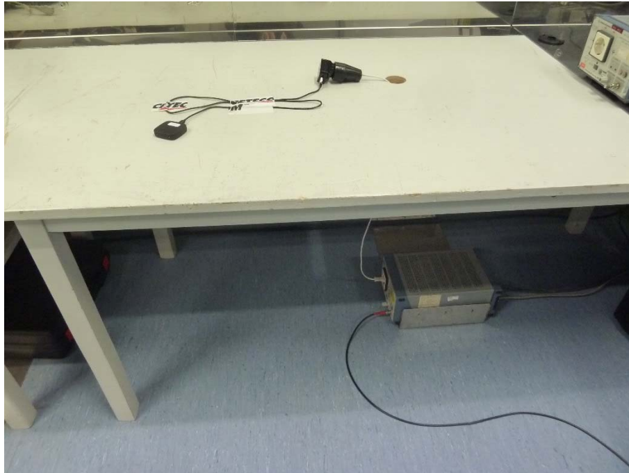
Photo 7: AC conducted test setup
