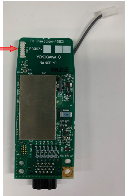
Figure 2. Antenna location
