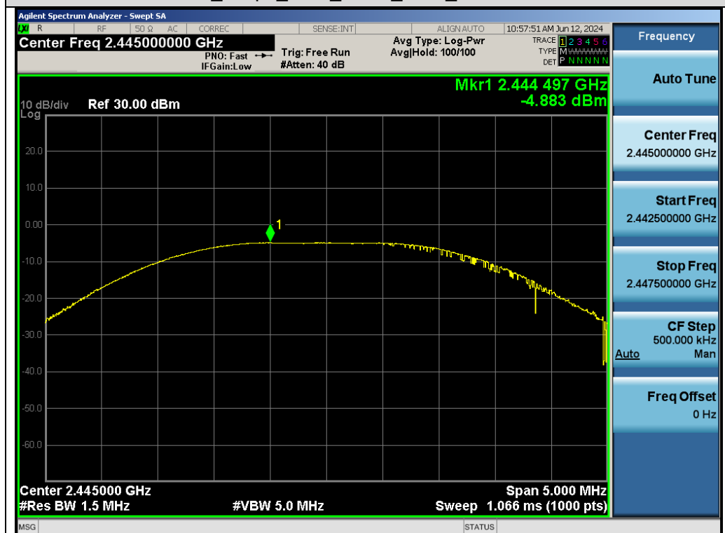
Test_Graph_2.4G_ANT1_2445_Peak Power
