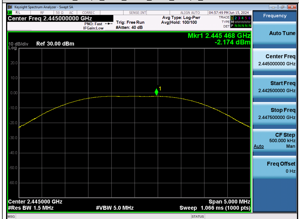
Test_Graph_2.4G_ANT1_2445_2Mbps_Peak Power
