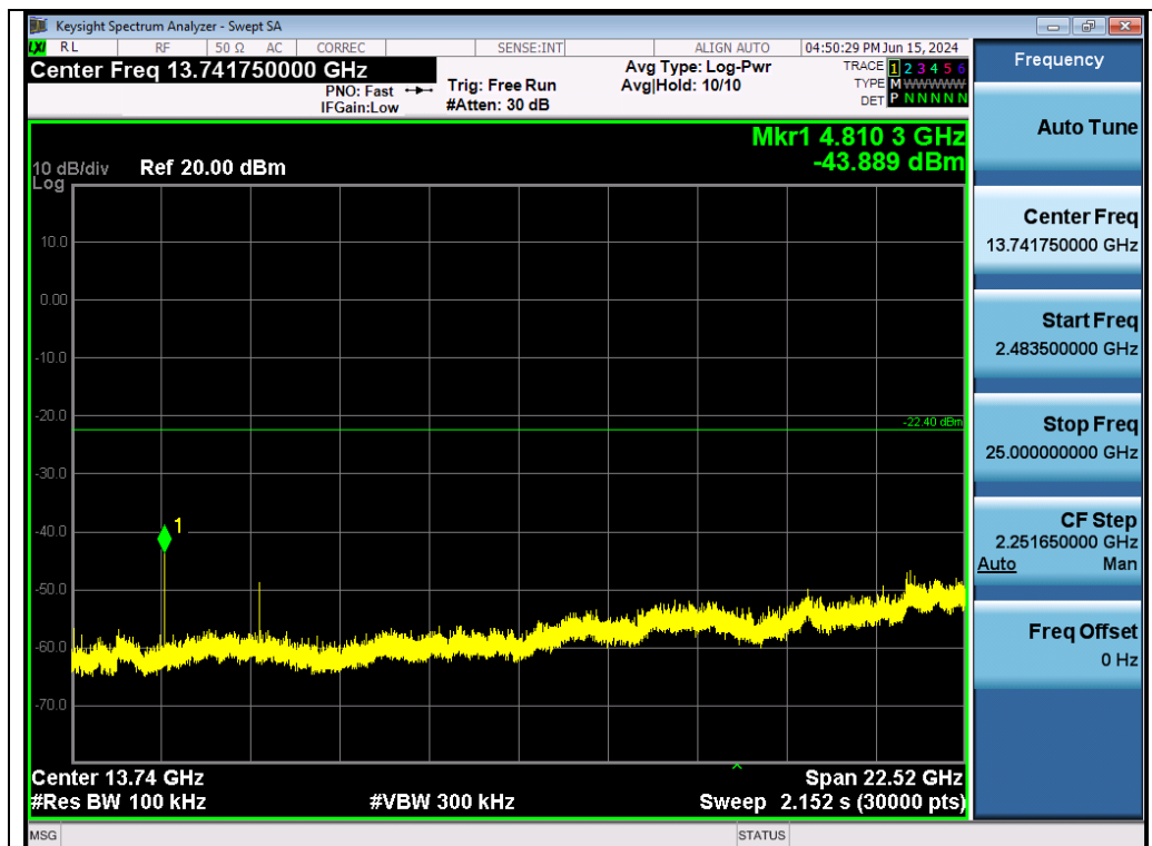
Test_Graph_2.4G_ANT1_2405_2Mbps_Higher Band Emissions
