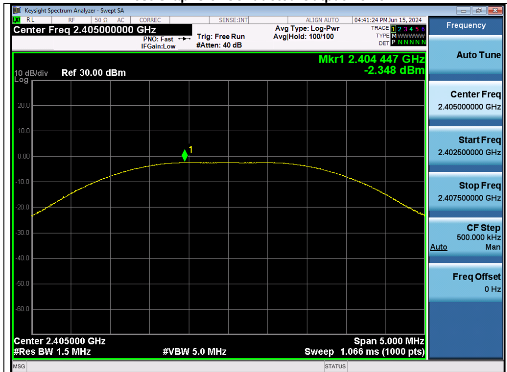
Test_Graph_2.4G_ANT1_2405_2Mbps_Peak Power
