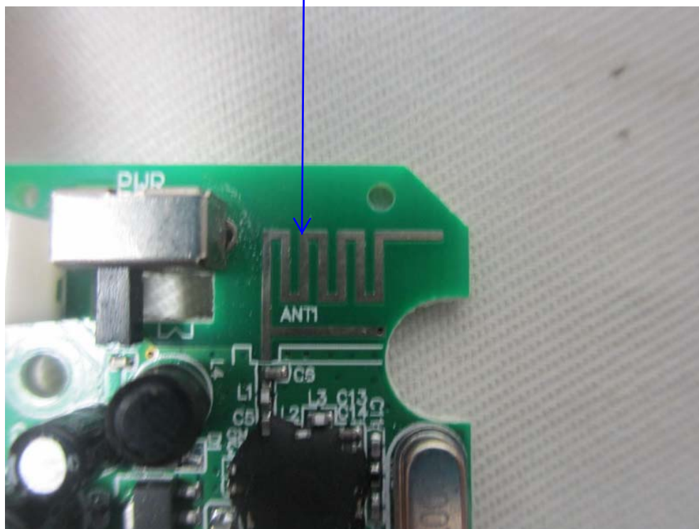
Printed antenna
