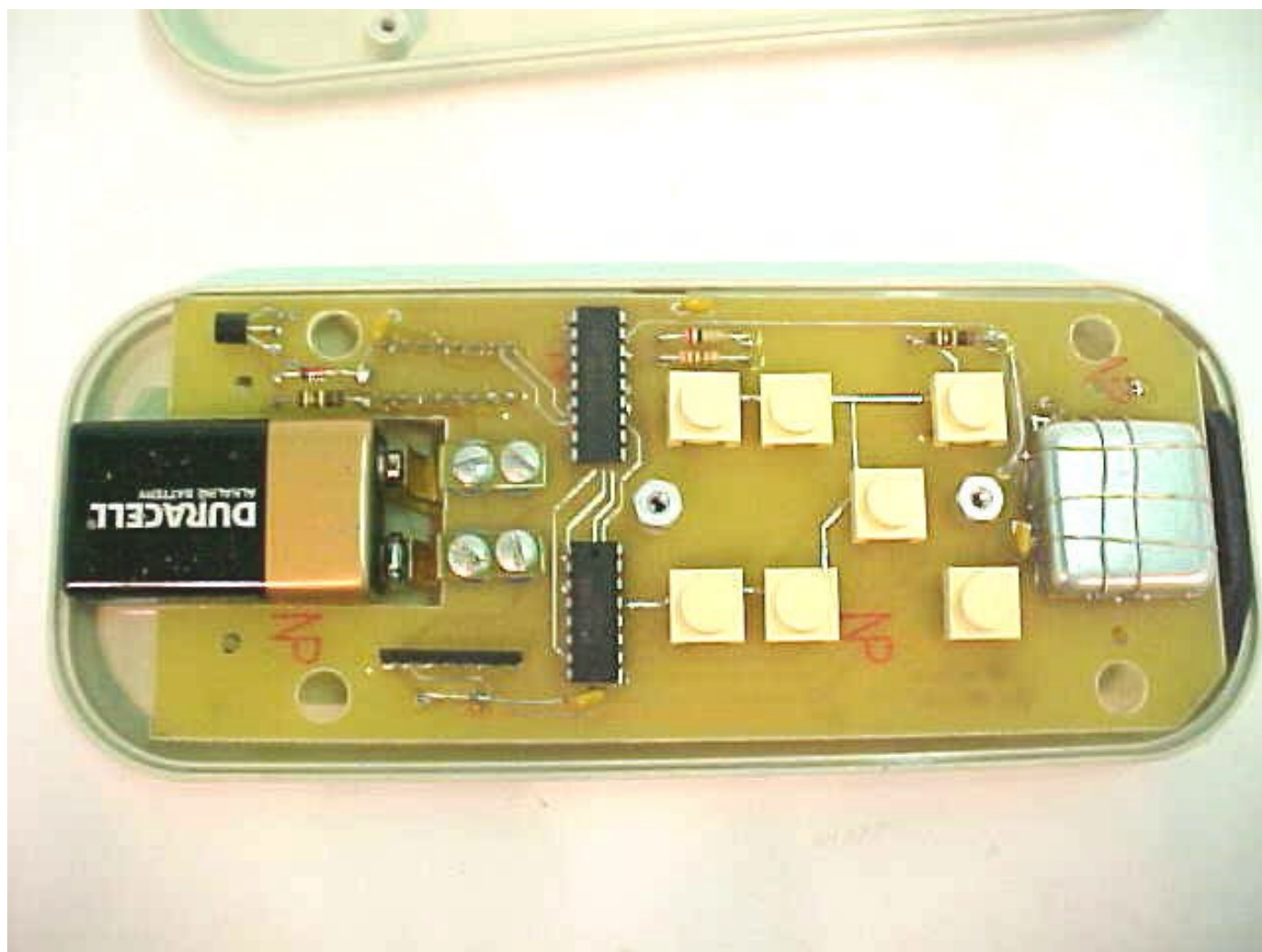
EUT Internal Front
