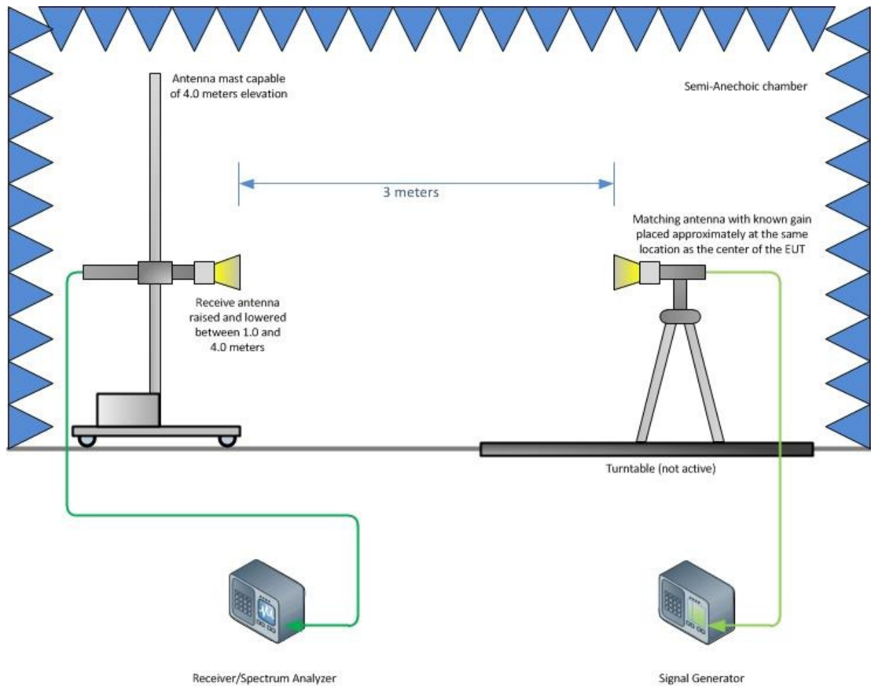
Substitution Test Method (Above 1GHz, if applicable)
