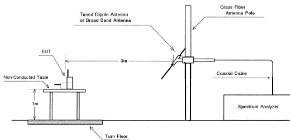
Test setup in an anechoic chamber
