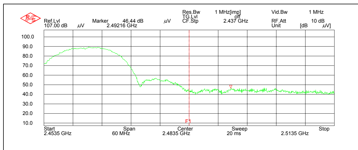
Figure 7.6.3.2-1: Band Edge CAP – Peak
