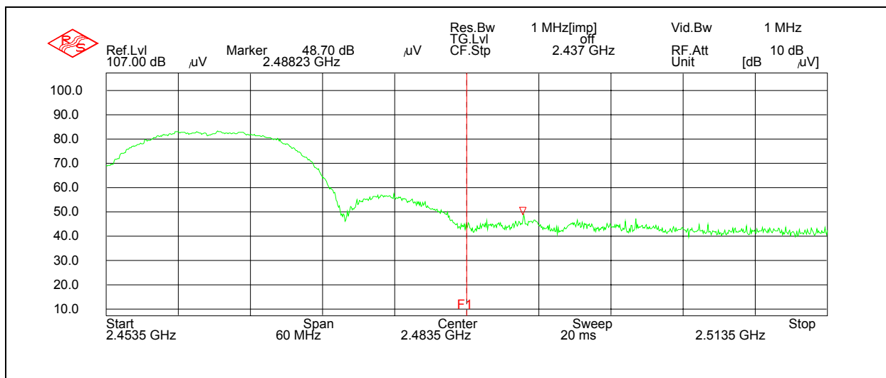
Figure 7.6.3.2-3: Band Edge WAB – Peak
