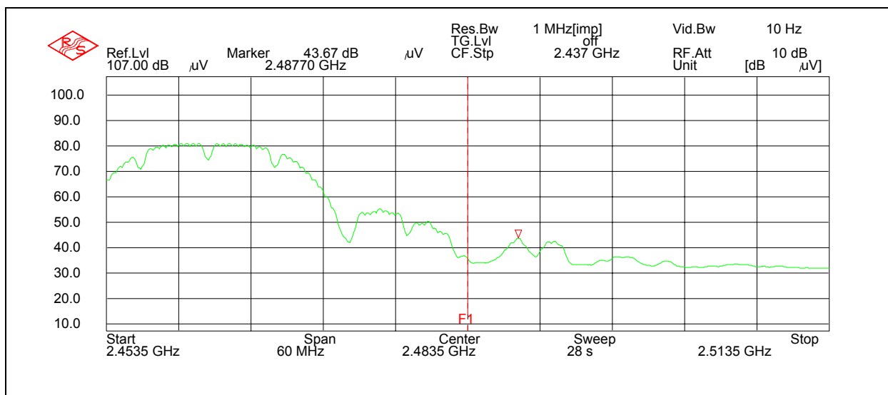
Figure 7.6.3.2-4: Band Edge WAB - Average
