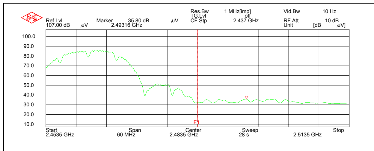
Figure 7.6.3.2-2: Band Edge CAP - Average
