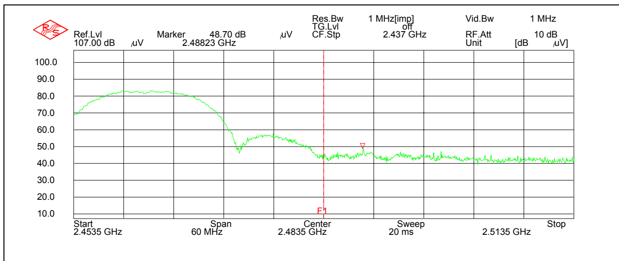
Figure 7.6.3-3: Band Edge WAB - Peak
