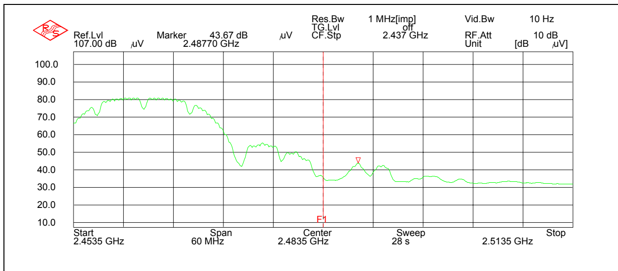
Figure 7.6.3-4: Band Edge WAB - Average
