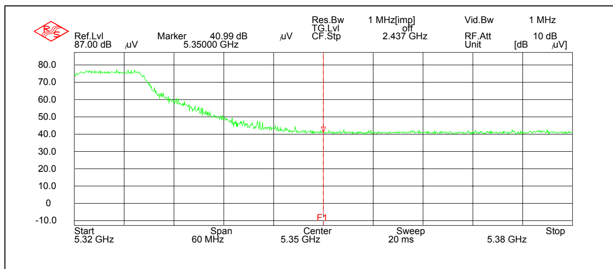
Figure 8.6.4-3: Band Edge Restricted Bands – Channel 64 – Peak
