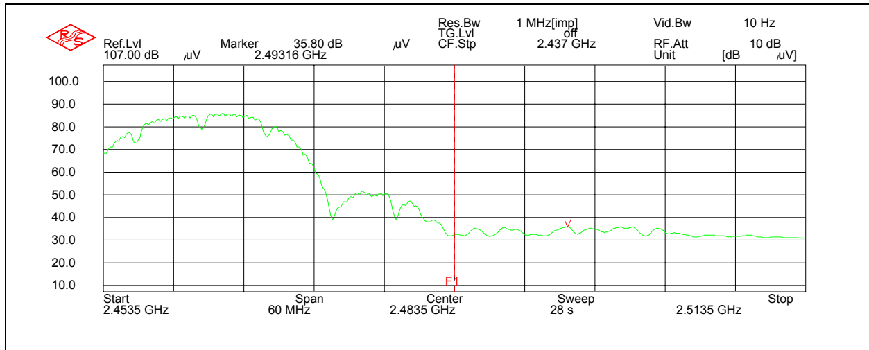
Figure 7.6.3-2: Band Edge CAP - Average
