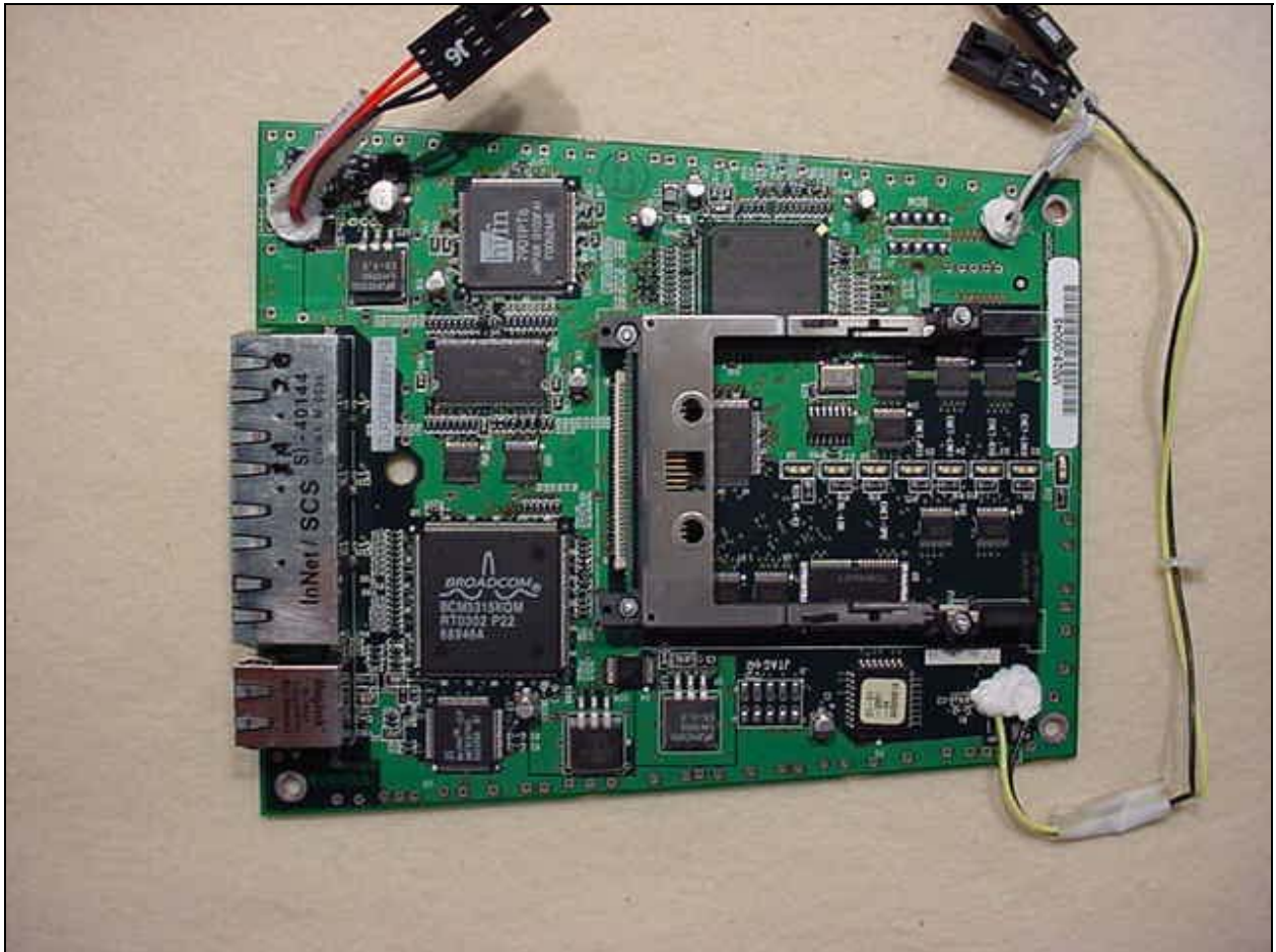
Figure 2: Internal – RF Board (Top View)
