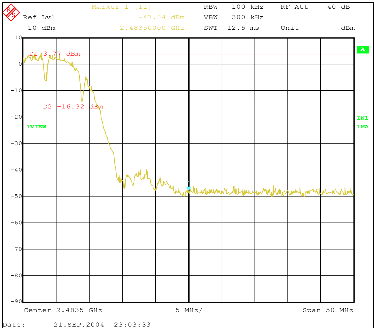
Figure 2: Upper Banedge
