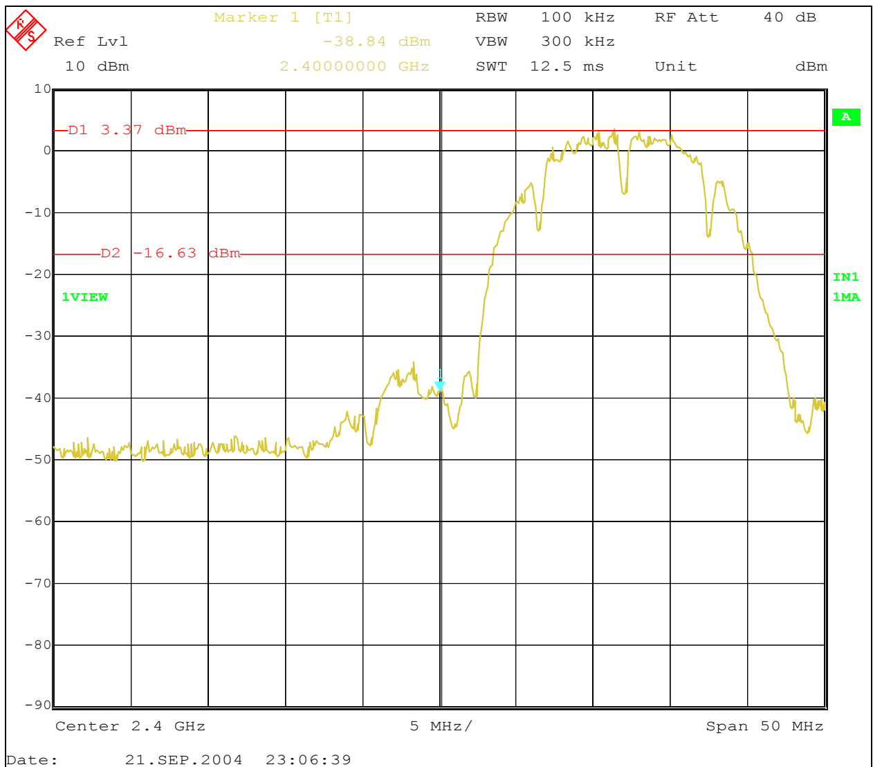
Figure 1: Lower Bandedge
