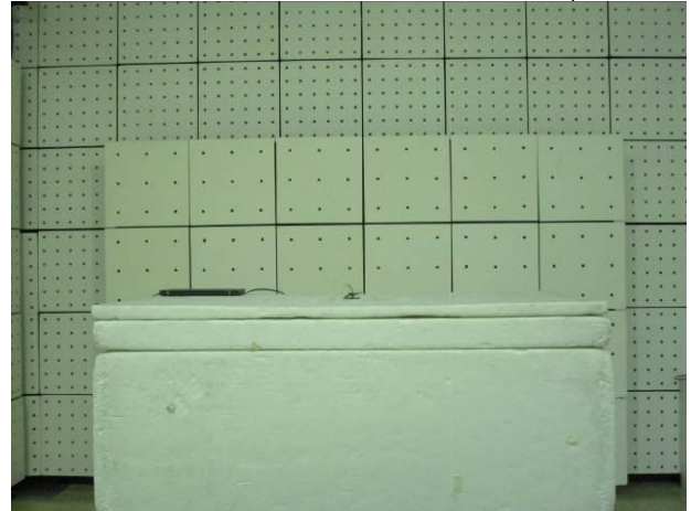
FCC_15_247_BLE_Radiated_AN54LQ-P_Setup
