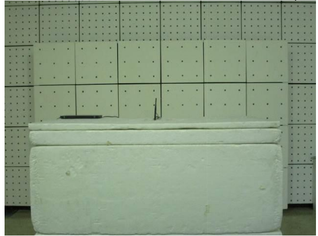
FCC 15_247+IC_RSS_247_BLE_Radiated_AN54LQ-U_Setup
