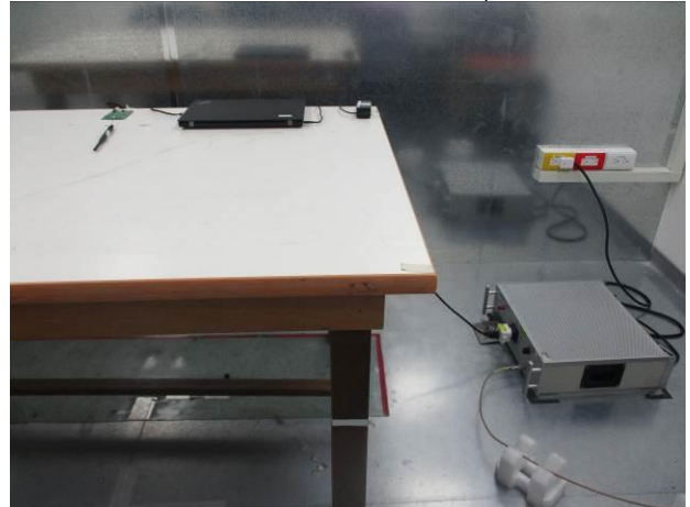
AN54LQ-U_Conduction_Setup
