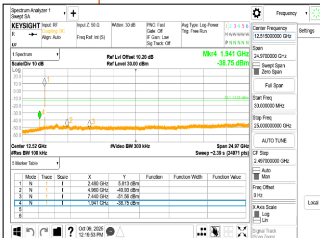
Spurious Emission_BLE 1M_HighCH39-2480MHz
