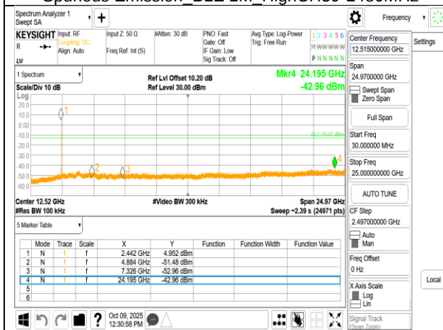
Spurious Emission_BLE 2M_MidCH20-2442MHz
