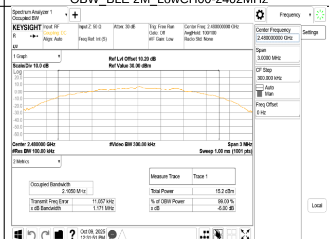
OBW_BLE 2M_HighCH39-2480MHz
