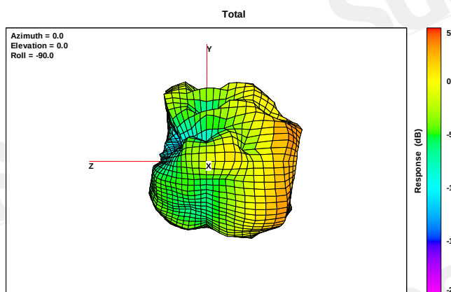
Free Space EIRP (5290 MHz) - 3D
