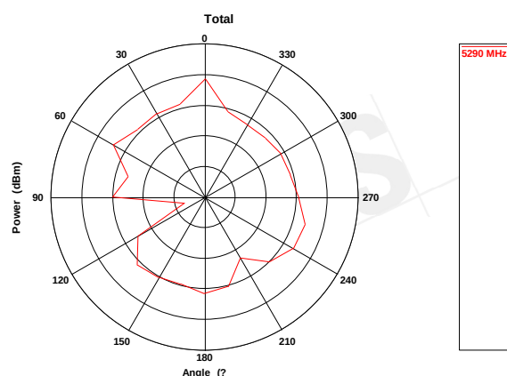
Free Space EIRP (5290 MHz) - XY cut
