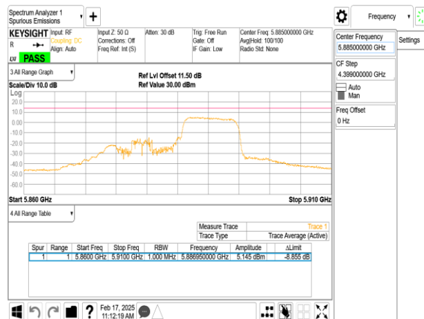
802.11ax_20MHz_Chain0_5885MHz_RU106_54
